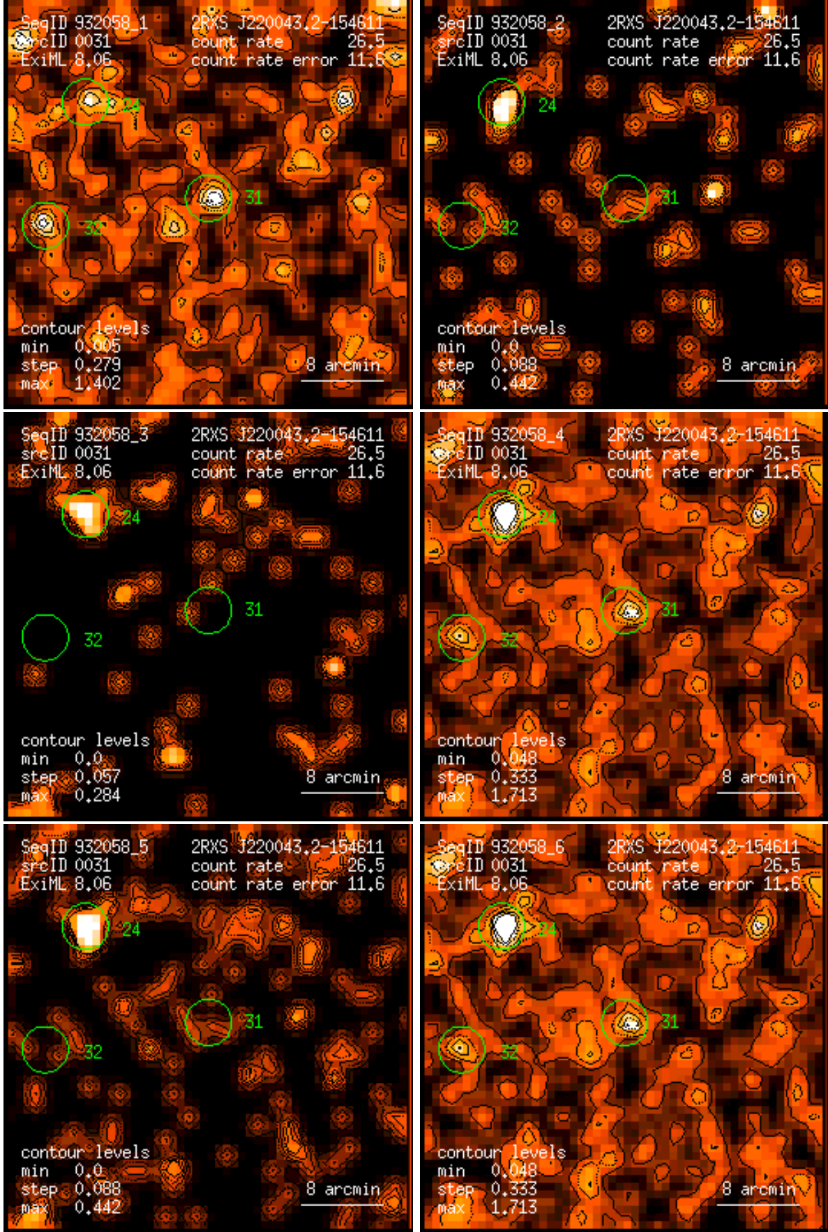
Figure 31: RASS 932058: detection 0031: band rate images, Gaussian filter: (1) PSPC channels 11 – 41, (2) 52 – 90, (3) 91 – 201, (4) 11 – 235, (5) 52 – 201, (6) 11 – 201. Broad band rates in counts/ks. Band rate contour levels in counts/ks/arcmin 2 .
