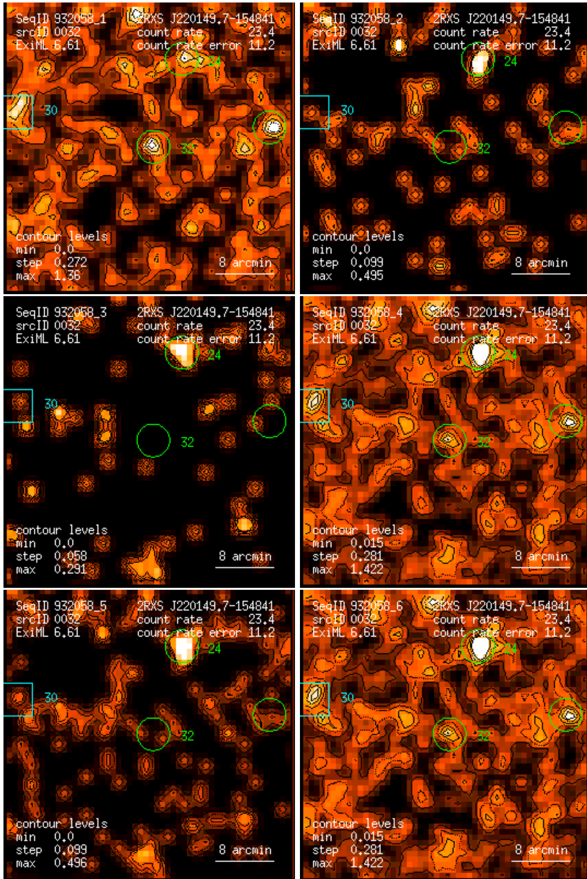
Figure 32: RASS 932058: detection 0032: band rate images, Gaussian filter: (1) PSPC channels 11 – 41, (2) 52 – 90, (3) 91 – 201, (4) 11 – 235, (5) 52 – 201, (6) 11 – 201. Broad band rates in counts/ks. Band rate contour levels in counts/ks/arcmin 2 .
