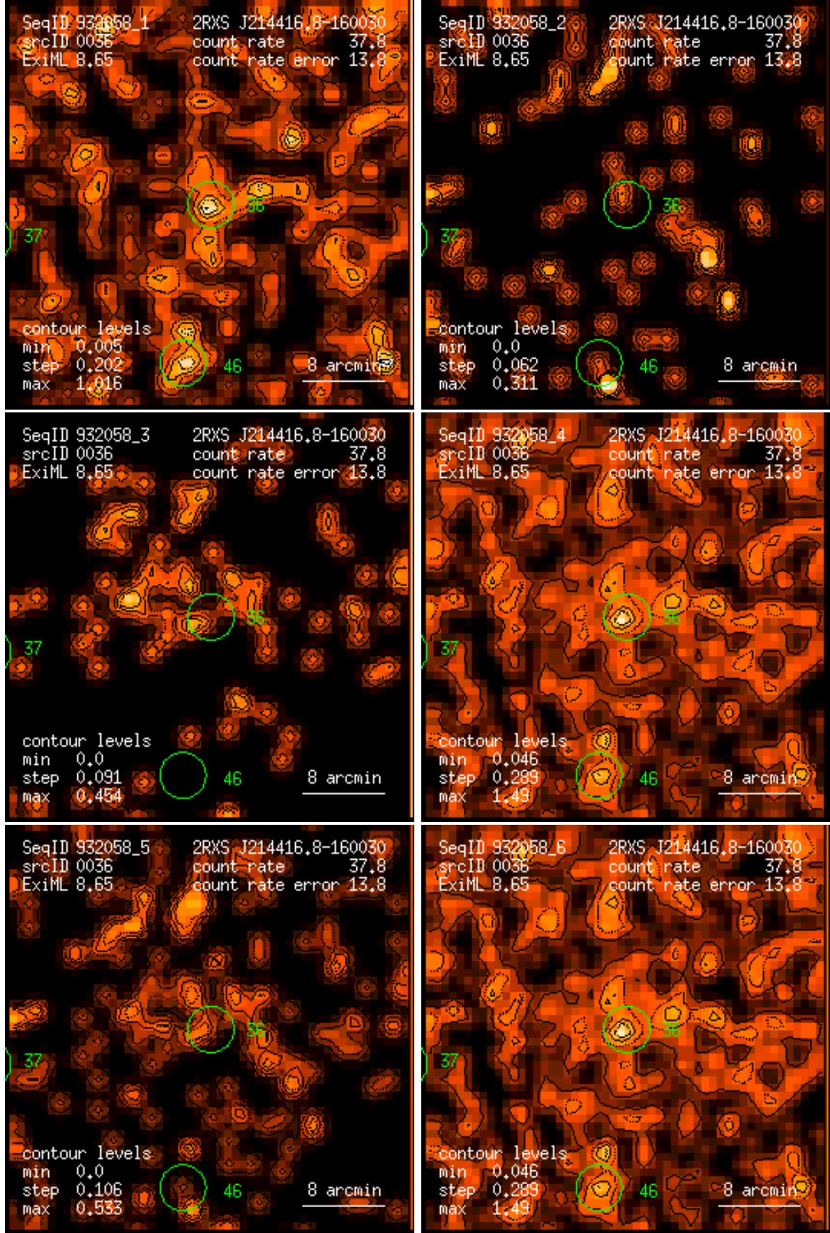
Figure 36: RASS 932058: detection 0036: band rate images, Gaussian filter: (1) PSPC channels 11 – 41, (2) 52 – 90, (3) 91 – 201, (4) 11 – 235, (5) 52 – 201, (6) 11 – 201. Broad band rates in counts/ks. Band rate contour levels in counts/ks/arcmin 2 .
