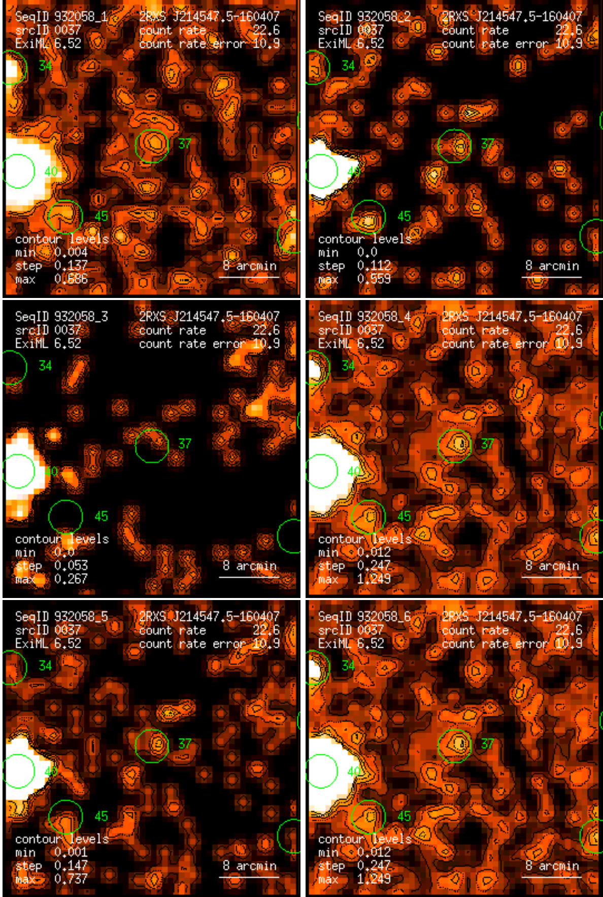
Figure 37: RASS 932058: detection 0037: band rate images, Gaussian filter: (1) PSPC channels 11 – 41, (2) 52 – 90, (3) 91 – 201, (4) 11 – 235, (5) 52 – 201, (6) 11 – 201. Broad band rates in counts/ks. Band rate contour levels in counts/ks/arcmin 2 .
