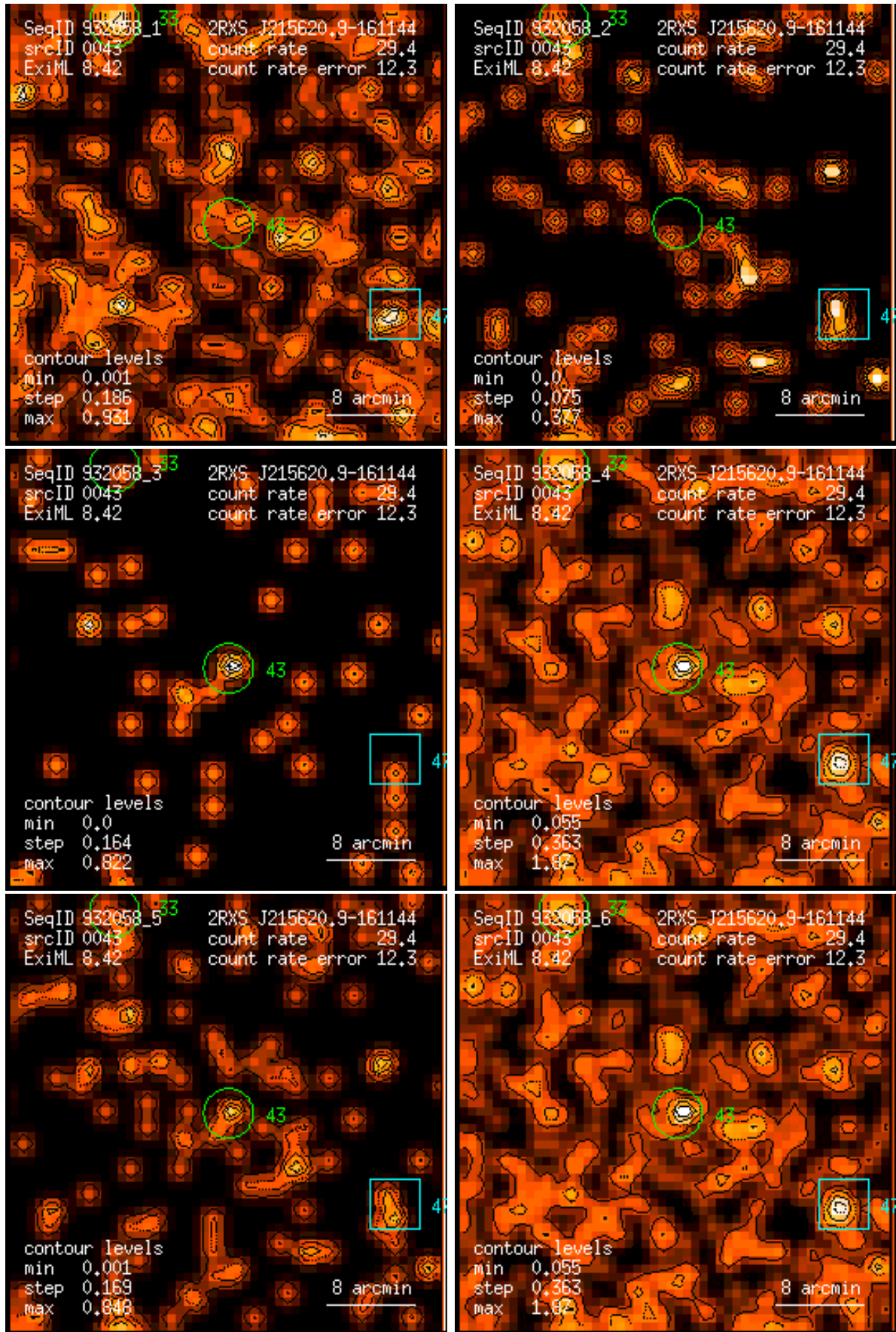
Figure 43: RASS 932058: detection 0043: band rate images, Gaussian filter: (1) PSPC channels 11 – 41, (2) 52 – 90, (3) 91 – 201, (4) 11 – 235, (5) 52 – 201, (6) 11 – 201. Broad band rates in counts/ks. Band rate contour levels in counts/ks/arcmin 2 .
