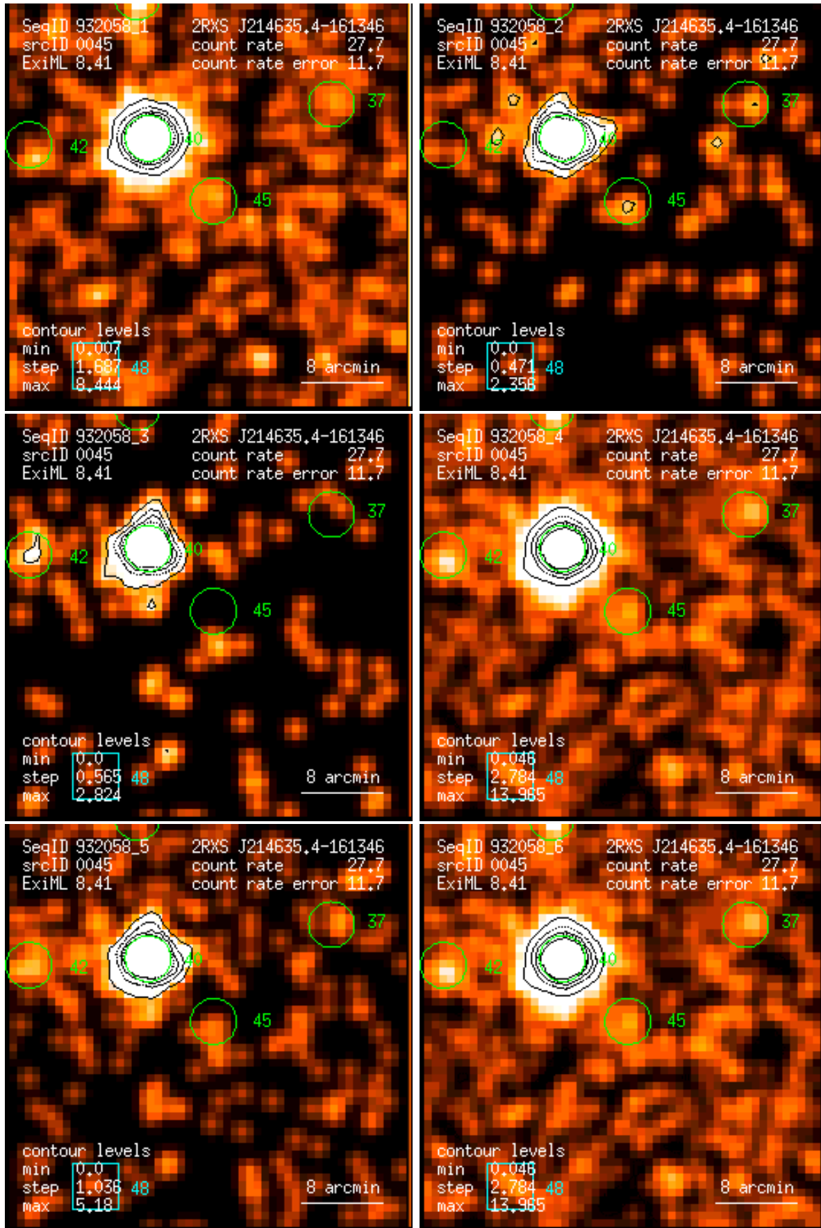
Figure 45: RASS 932058: detection 0045: band rate images, Gaussian filter: (1) PSPC channels 11 – 41, (2) 52 – 90, (3) 91 – 201, (4) 11 – 235, (5) 52 – 201, (6) 11 – 201. Broad band rates in counts/ks. Band rate contour levels in counts/ks/arcmin 2 .
