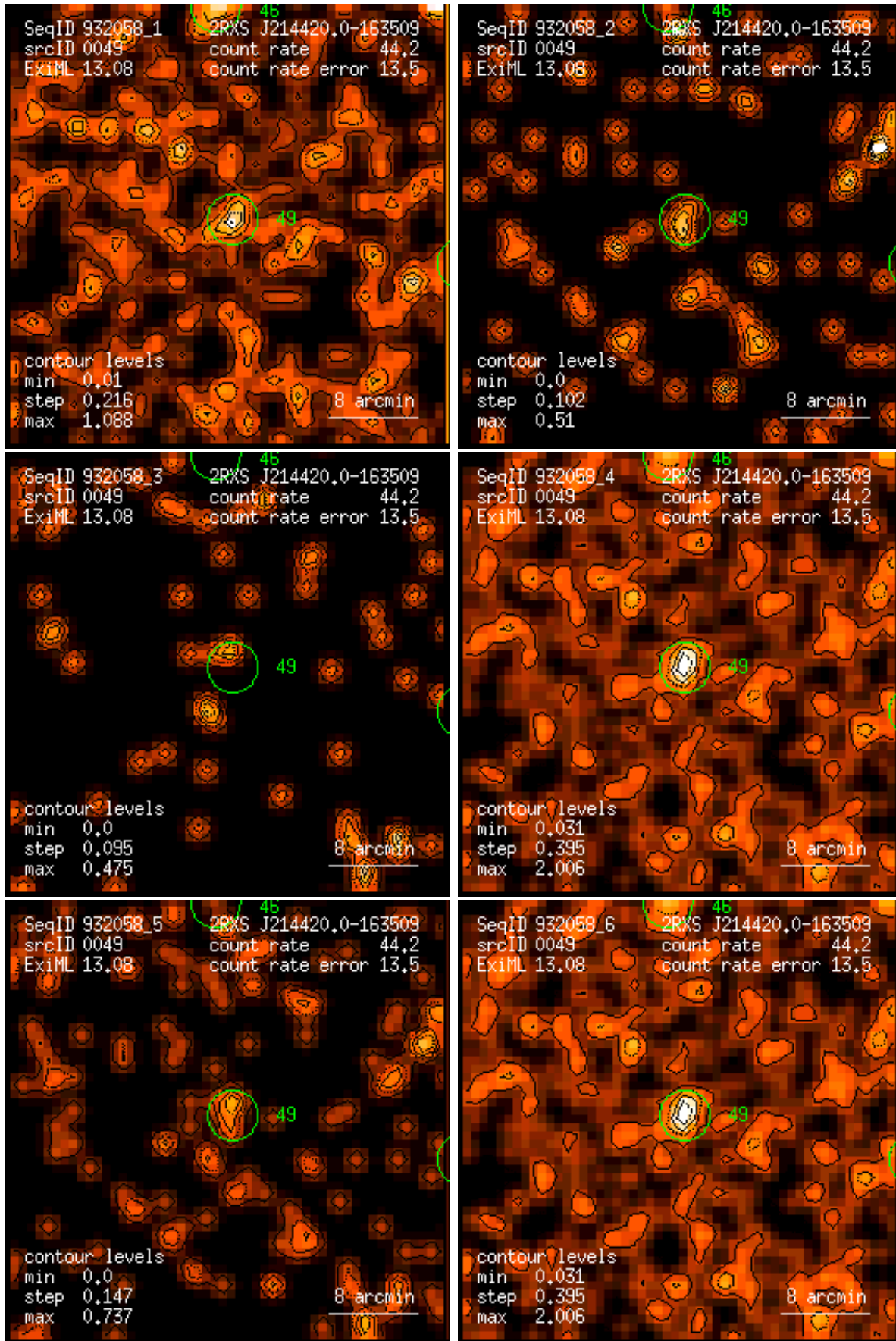
Figure 49: RASS 932058: detection 0049: band rate images, Gaussian filter: (1) PSPC channels 11 – 41, (2) 52 – 90, (3) 91 – 201, (4) 11 – 235, (5) 52 – 201, (6) 11 – 201. Broad band rates in counts/ks. Band rate contour levels in counts/ks/arcmin 2 .
