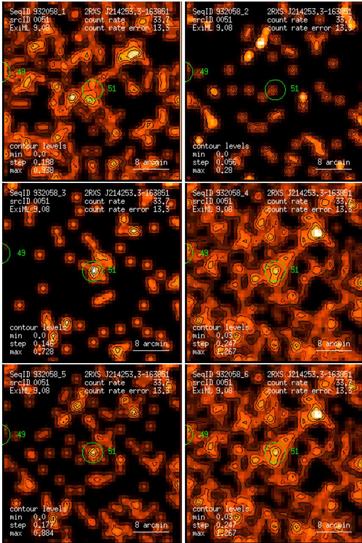
Figure 51: RASS 932058: detection 0051: band rate images, Gaussian filter: (1) PSPC channels 11 – 41, (2) 52 – 90, (3) 91 – 201, (4) 11 – 235, (5) 52 – 201, (6) 11 – 201. Broad band rates in counts/ks. Band rate contour levels in counts/ks/arcmin 2 .
