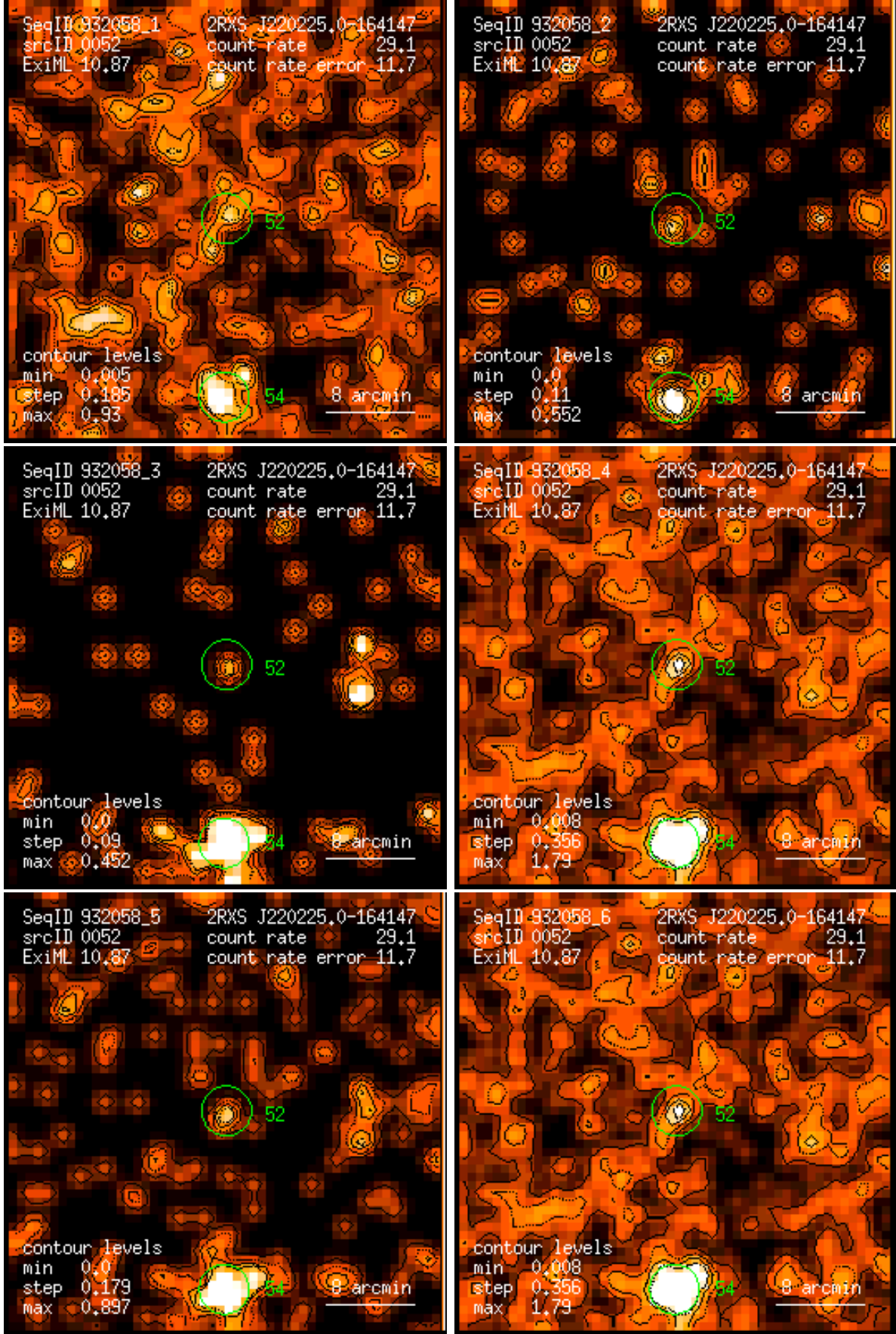
Figure 52: RASS 932058: detection 0052: band rate images, Gaussian filter: (1) PSPC channels 11 – 41, (2) 52 – 90, (3) 91 – 201, (4) 11 – 235, (5) 52 – 201, (6) 11 – 201. Broad band rates in counts/ks. Band rate contour levels in counts/ks/arcmin 2 .
