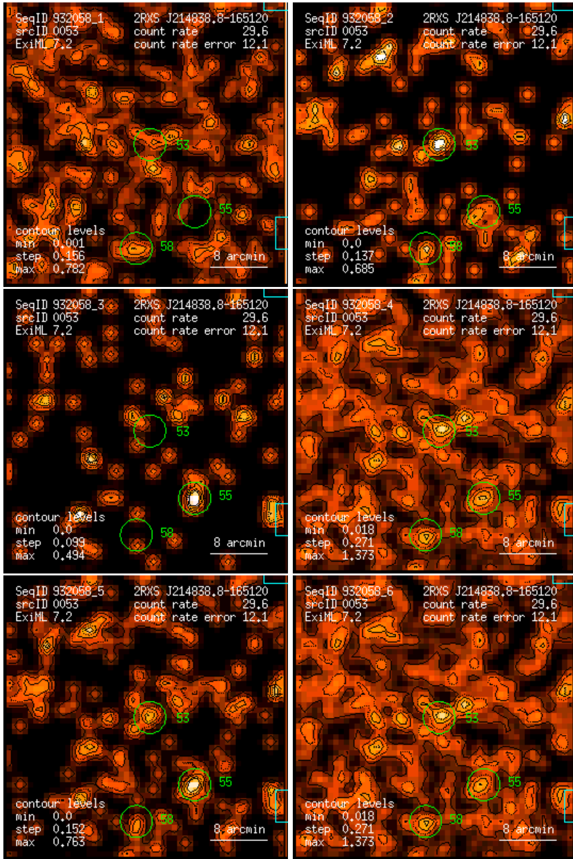
Figure 53: RASS 932058: detection 0053: band rate images, Gaussian filter: (1) PSPC channels 11 – 41, (2) 52 – 90, (3) 91 – 201, (4) 11 – 235, (5) 52 – 201, (6) 11 – 201. Broad band rates in counts/ks. Band rate contour levels in counts/ks/arcmin 2 .
