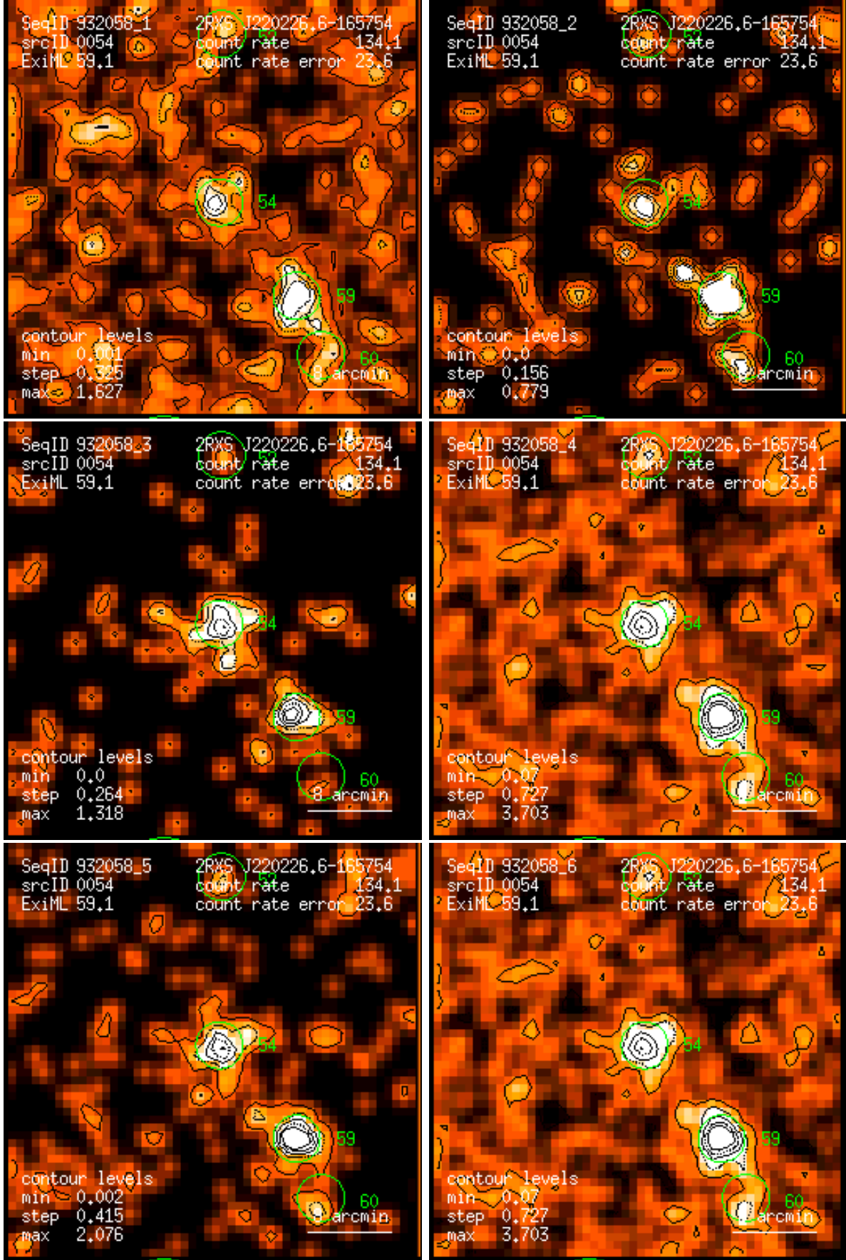
Figure 54: RASS 932058: detection 0054: band rate images, Gaussian filter: (1) PSPC channels 11 – 41, (2) 52 – 90, (3) 91 – 201, (4) 11 – 235, (5) 52 – 201, (6) 11 – 201. Broad band rates in counts/ks. Band rate contour levels in counts/ks/arcmin 2 .
