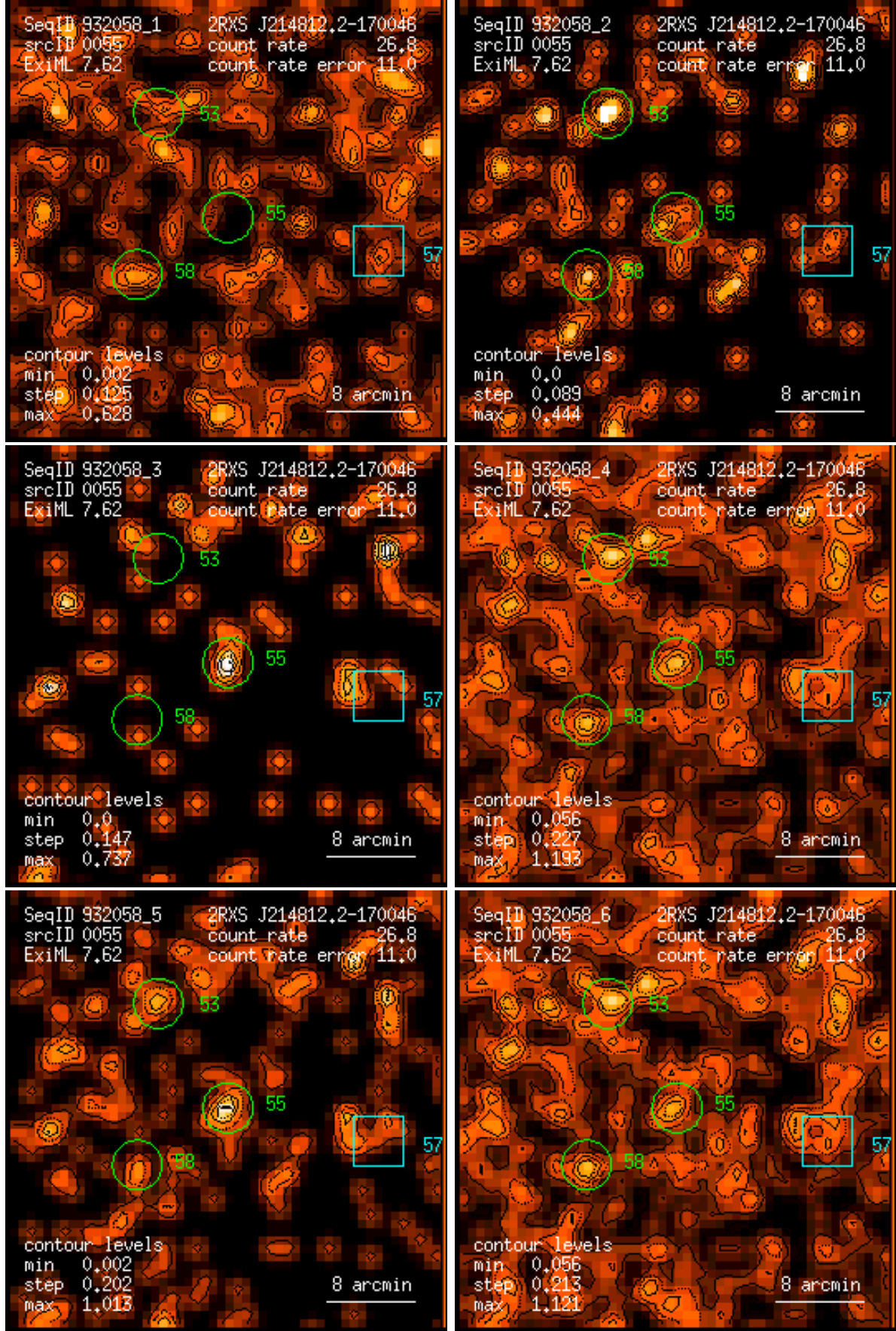
Figure 55: RASS 932058: detection 0055: band rate images, Gaussian filter: (1) PSPC channels 11 – 41, (2) 52 – 90, (3) 91 – 201, (4) 11 – 235, (5) 52 – 201, (6) 11 – 201. Broad band rates in counts/ks. Band rate contour levels in counts/ks/arcmin 2 .
