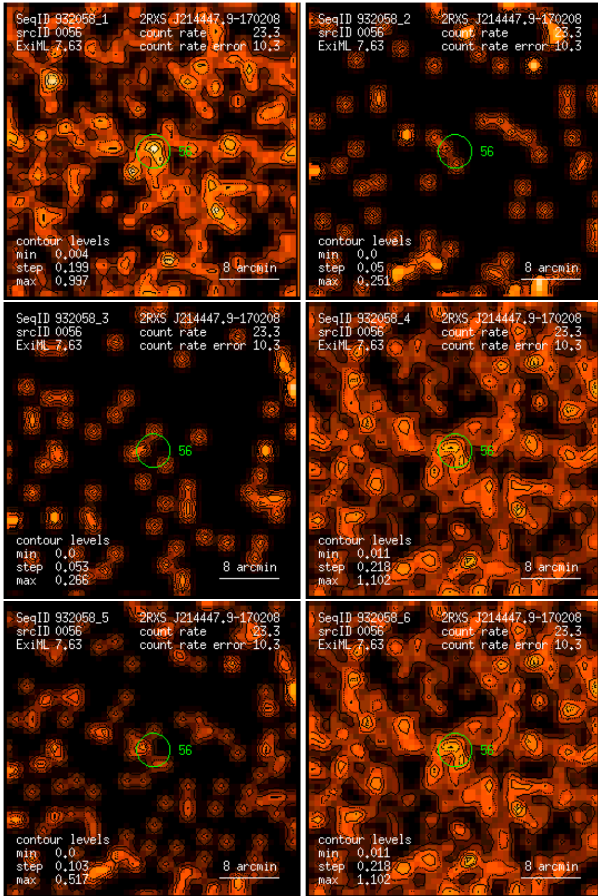
Figure 56: RASS 932058: detection 0056: band rate images, Gaussian filter: (1) PSPC channels 11 – 41, (2) 52 – 90, (3) 91 – 201, (4) 11 – 235, (5) 52 – 201, (6) 11 – 201. Broad band rates in counts/ks. Band rate contour levels in counts/ks/arcmin 2 .
