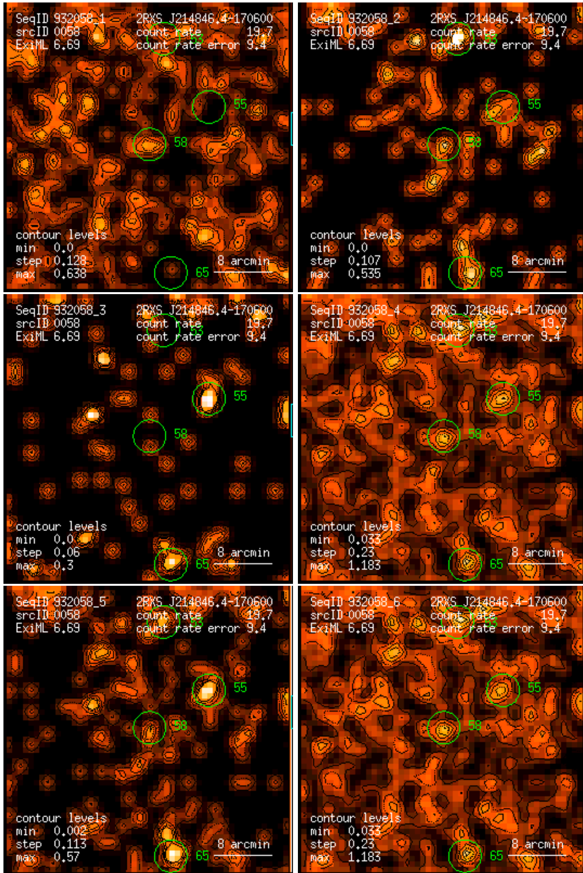
Figure 58: RASS 932058: detection 0058: band rate images, Gaussian filter: (1) PSPC channels 11 – 41, (2) 52 – 90, (3) 91 – 201, (4) 11 – 235, (5) 52 – 201, (6) 11 – 201. Broad band rates in counts/ks. Band rate contour levels in counts/ks/arcmin 2 .
