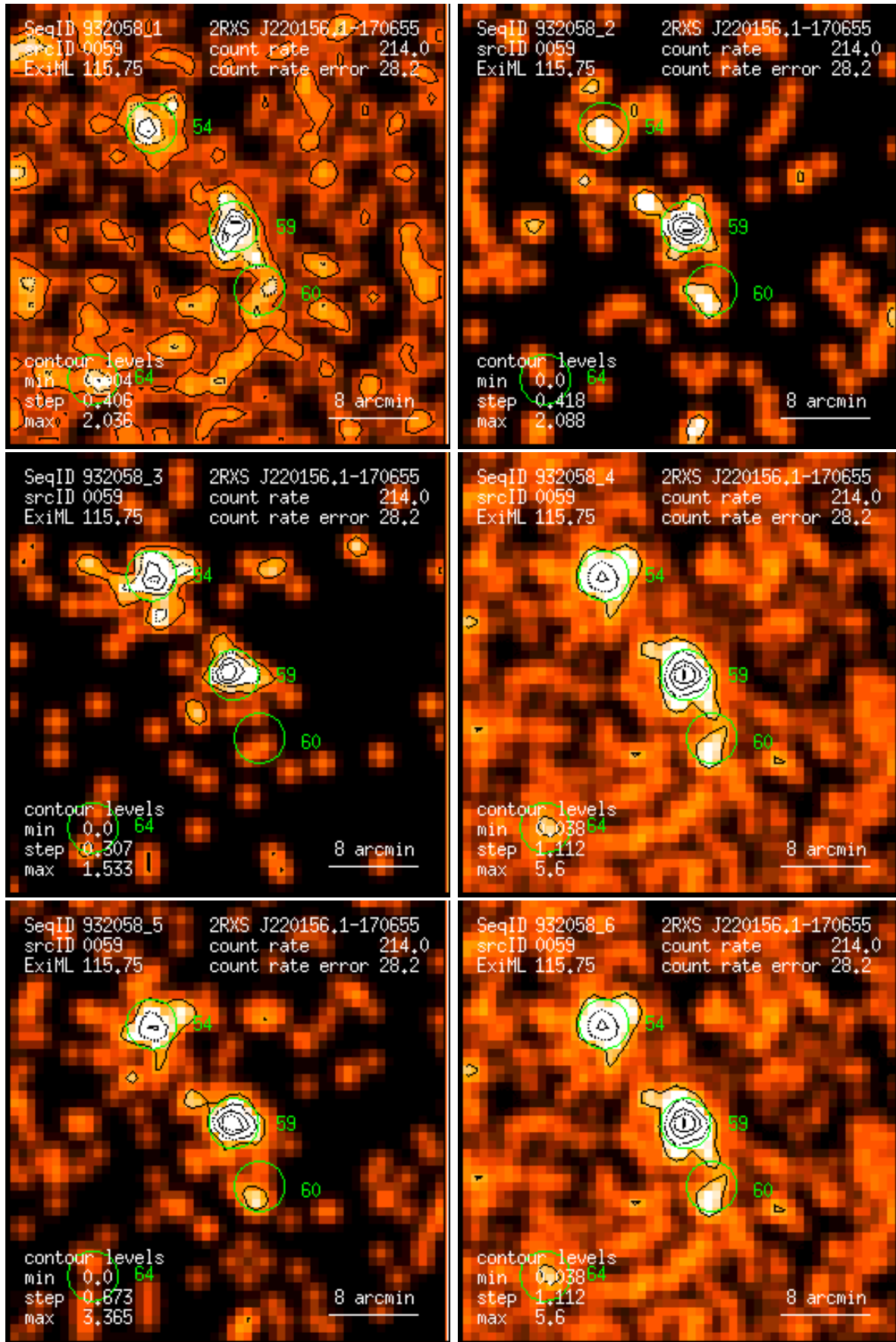
Figure 59: RASS 932058: detection 0059: band rate images, Gaussian filter: (1) PSPC channels 11 – 41, (2) 52 – 90, (3) 91 – 201, (4) 11 – 235, (5) 52 – 201, (6) 11 – 201. Broad band rates in counts/ks. Band rate contour levels in counts/ks/arcmin 2 .
