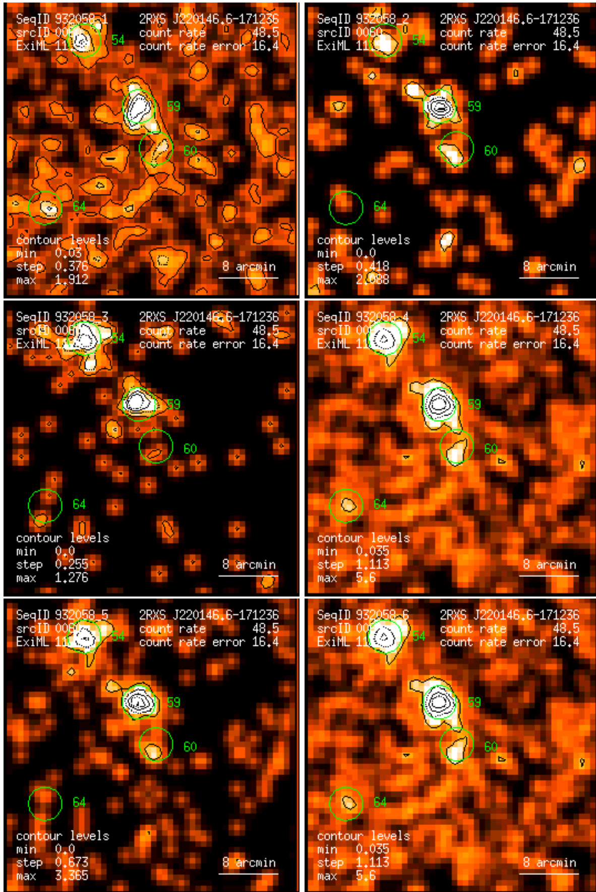
Figure 60: RASS 932058: detection 0060: band rate images, Gaussian filter: (1) PSPC channels 11 – 41, (2) 52 – 90, (3) 91 – 201, (4) 11 – 235, (5) 52 – 201, (6) 11 – 201. Broad band rates in counts/ks. Band rate contour levels in counts/ks/arcmin 2 .
