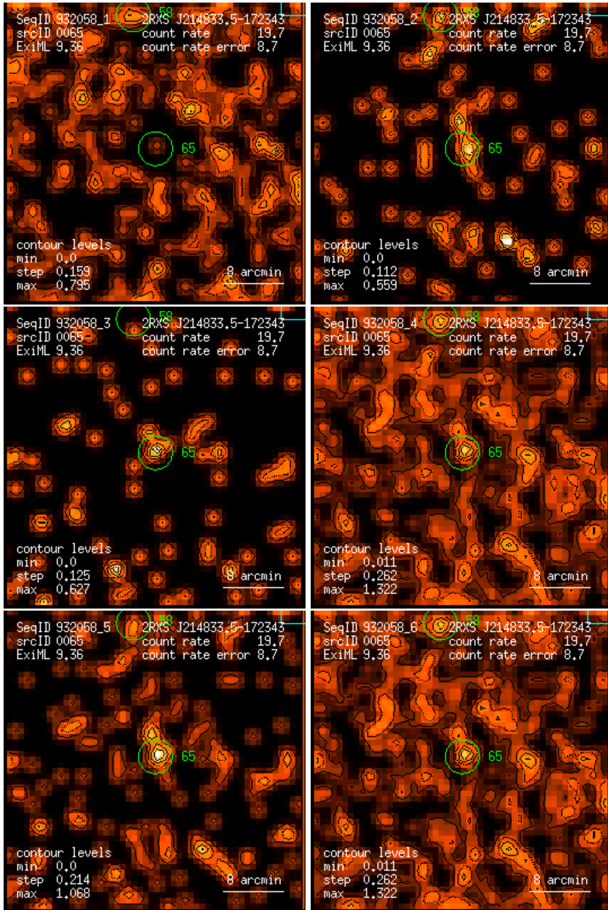
Figure 65: RASS 932058: detection 0065: band rate images, Gaussian filter: (1) PSPC channels 11 – 41, (2) 52 – 90, (3) 91 – 201, (4) 11 – 235, (5) 52 – 201, (6) 11 – 201. Broad band rates in counts/ks. Band rate contour levels in counts/ks/arcmin 2 .
