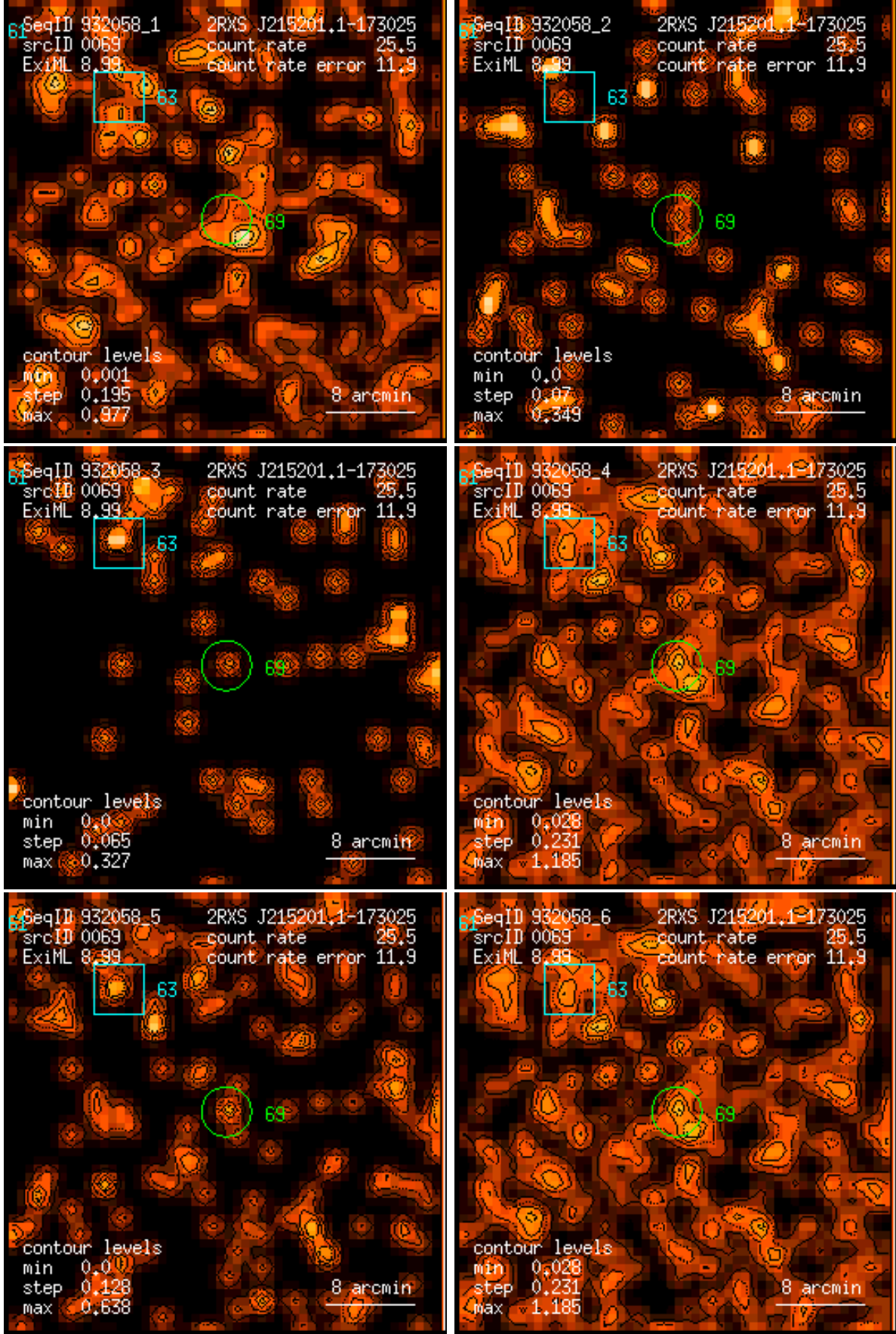
Figure 69: RASS 932058: detection 0069: band rate images, Gaussian filter: (1) PSPC channels 11 – 41, (2) 52 – 90, (3) 91 – 201, (4) 11 – 235, (5) 52 – 201, (6) 11 – 201. Broad band rates in counts/ks. Band rate contour levels in counts/ks/arcmin 2 .
