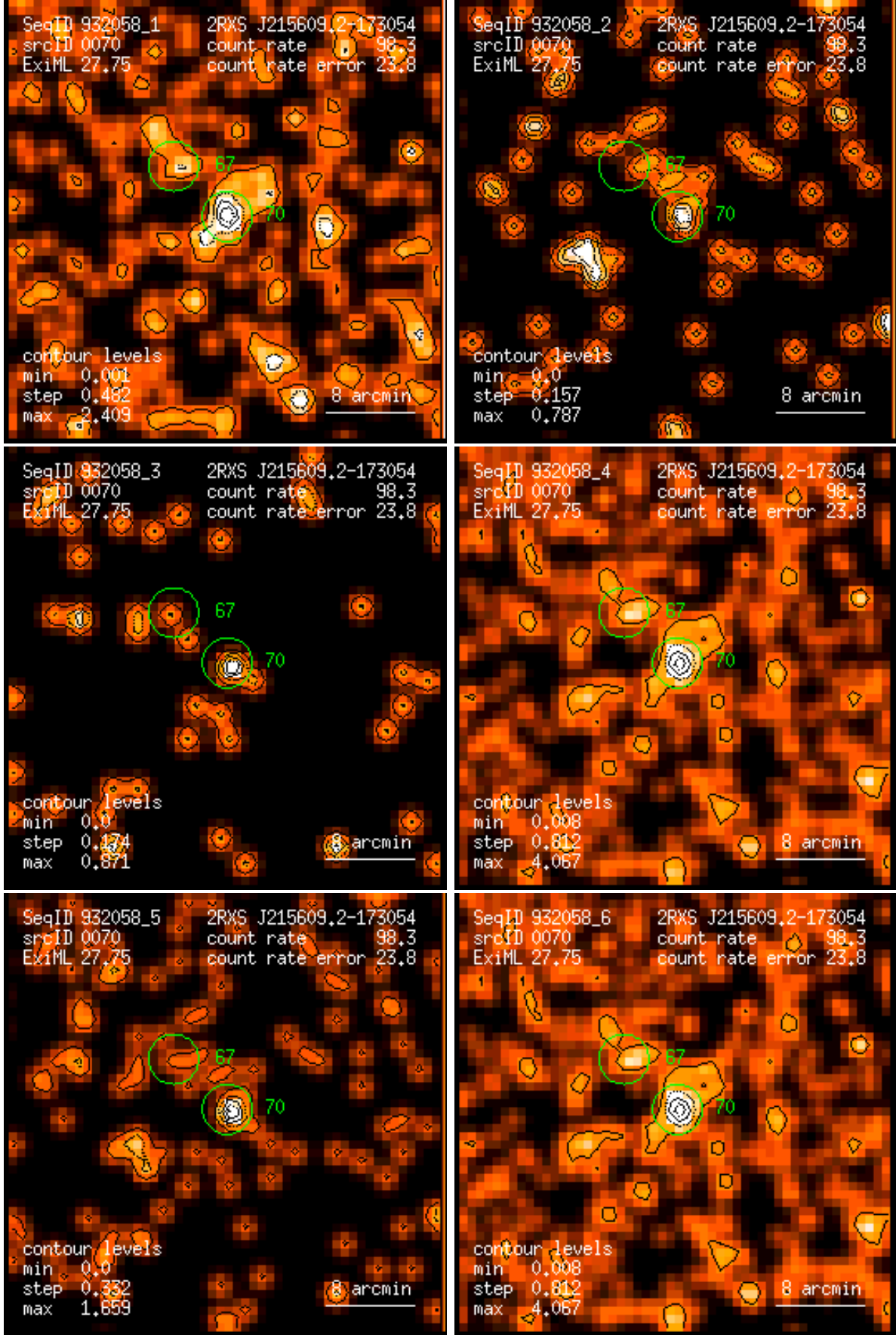
Figure 70: RASS 932058: detection 0070: band rate images, Gaussian filter: (1) PSPC channels 11 – 41, (2) 52 – 90, (3) 91 – 201, (4) 11 – 235, (5) 52 – 201, (6) 11 – 201. Broad band rates in counts/ks. Band rate contour levels in counts/ks/arcmin 2 .
