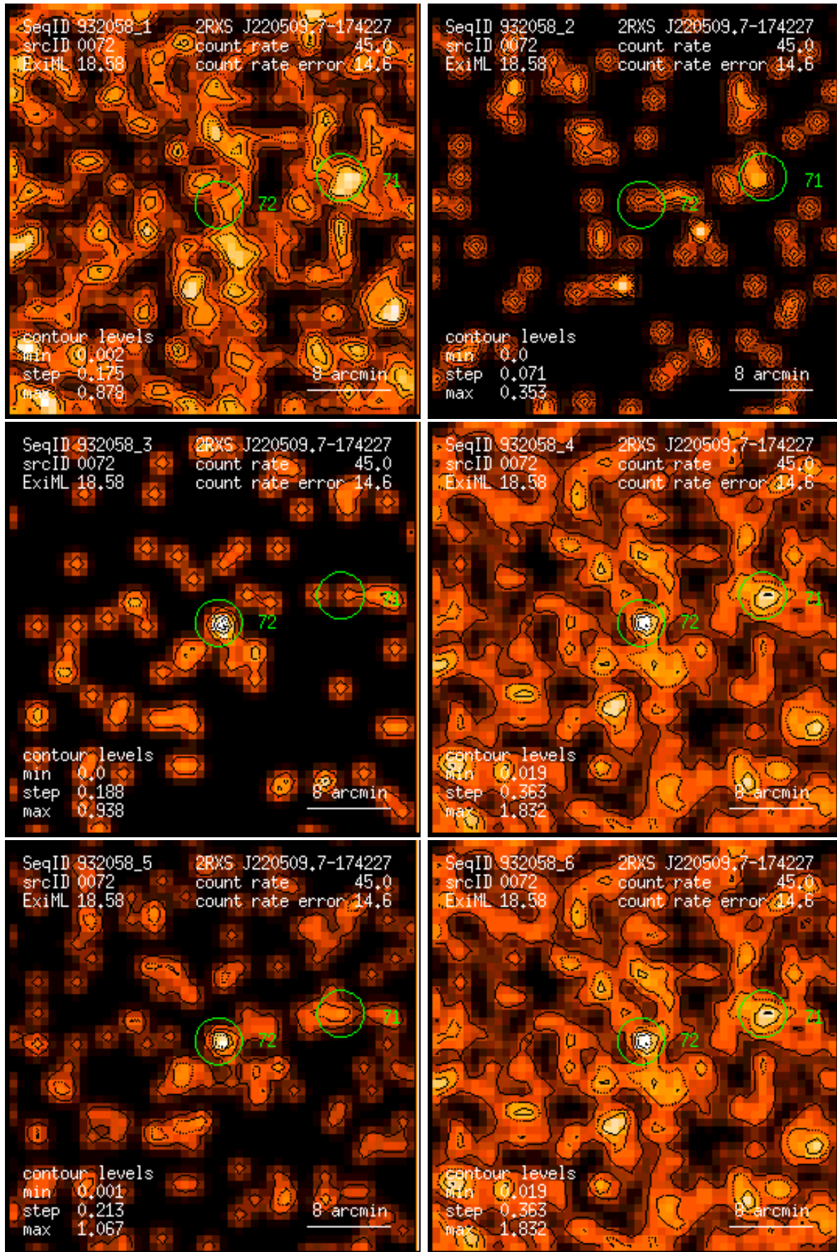
Figure 72: RASS 932058: detection 0072: band rate images, Gaussian filter: (1) PSPC channels 11 – 41, (2) 52 – 90, (3) 91 – 201, (4) 11 – 235, (5) 52 – 201, (6) 11 – 201. Broad band rates in counts/ks. Band rate contour levels in counts/ks/arcmin 2 .
