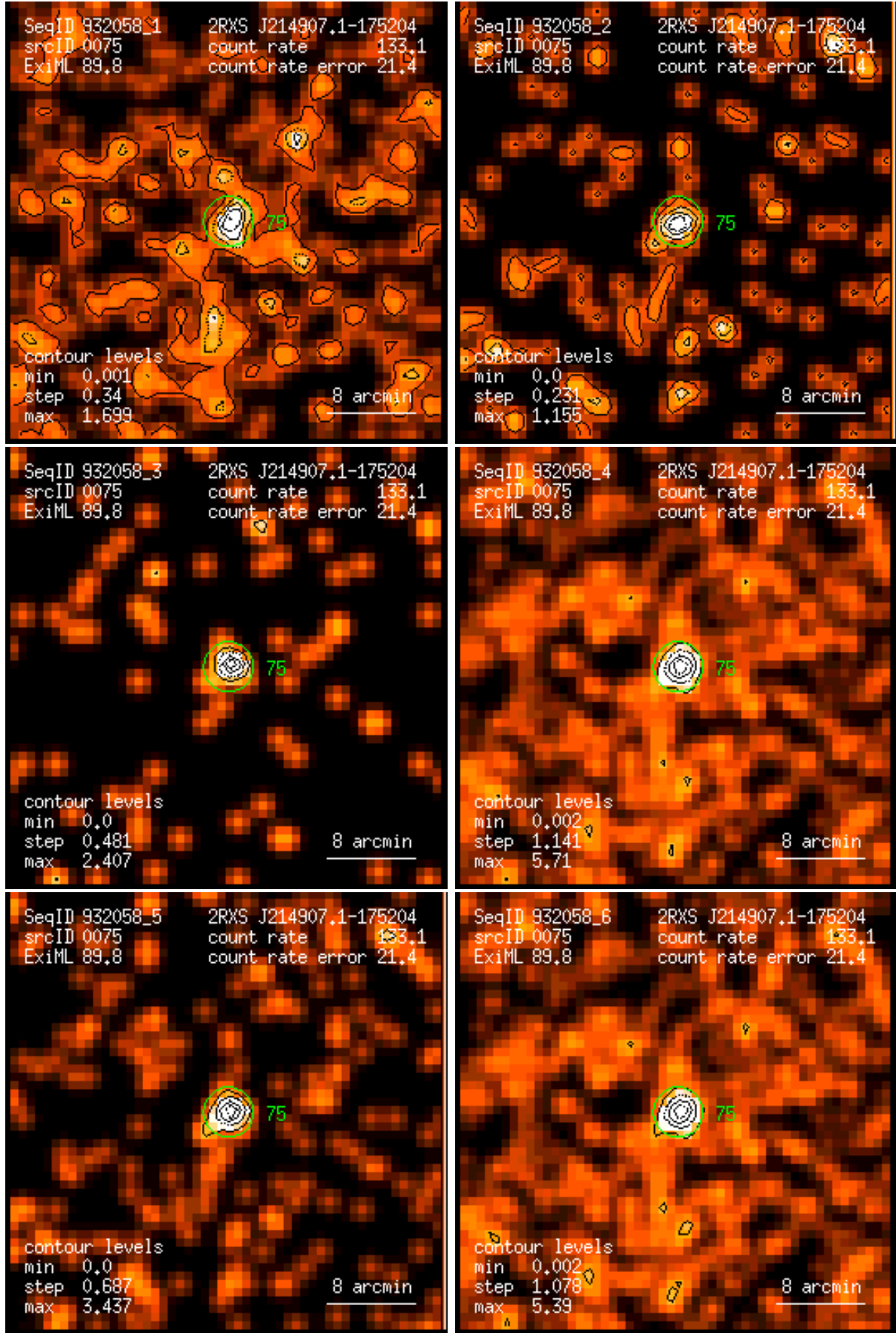
Figure 75: RASS 932058: detection 0075: band rate images, Gaussian filter: (1) PSPC channels 11 – 41, (2) 52 – 90, (3) 91 – 201, (4) 11 – 235, (5) 52 – 201, (6) 11 – 201. Broad band rates in counts/ks. Band rate contour levels in counts/ks/arcmin 2 .
