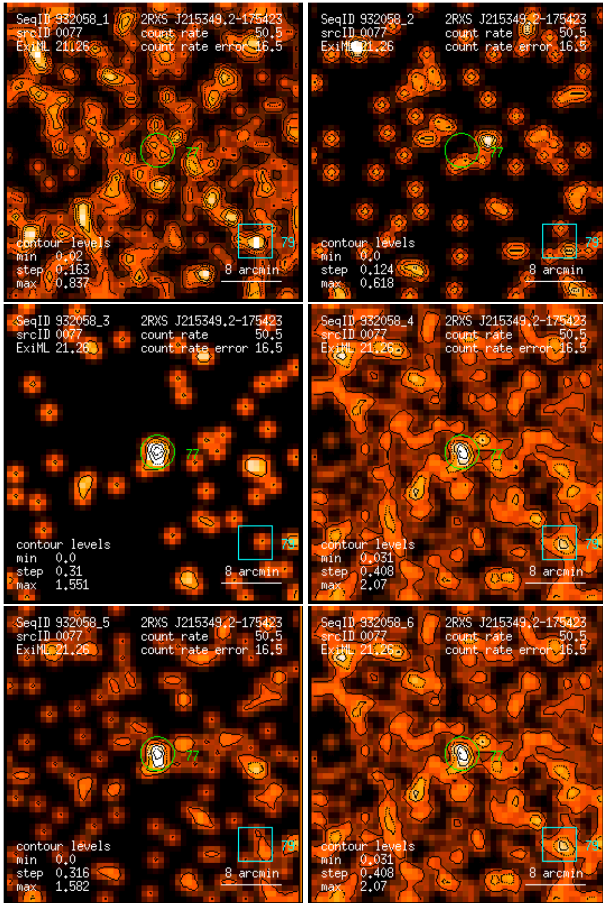
Figure 77: RASS 932058: detection 0077: band rate images, Gaussian filter: (1) PSPC channels 11 – 41, (2) 52 – 90, (3) 91 – 201, (4) 11 – 235, (5) 52 – 201, (6) 11 – 201. Broad band rates in counts/ks. Band rate contour levels in counts/ks/arcmin 2 .
