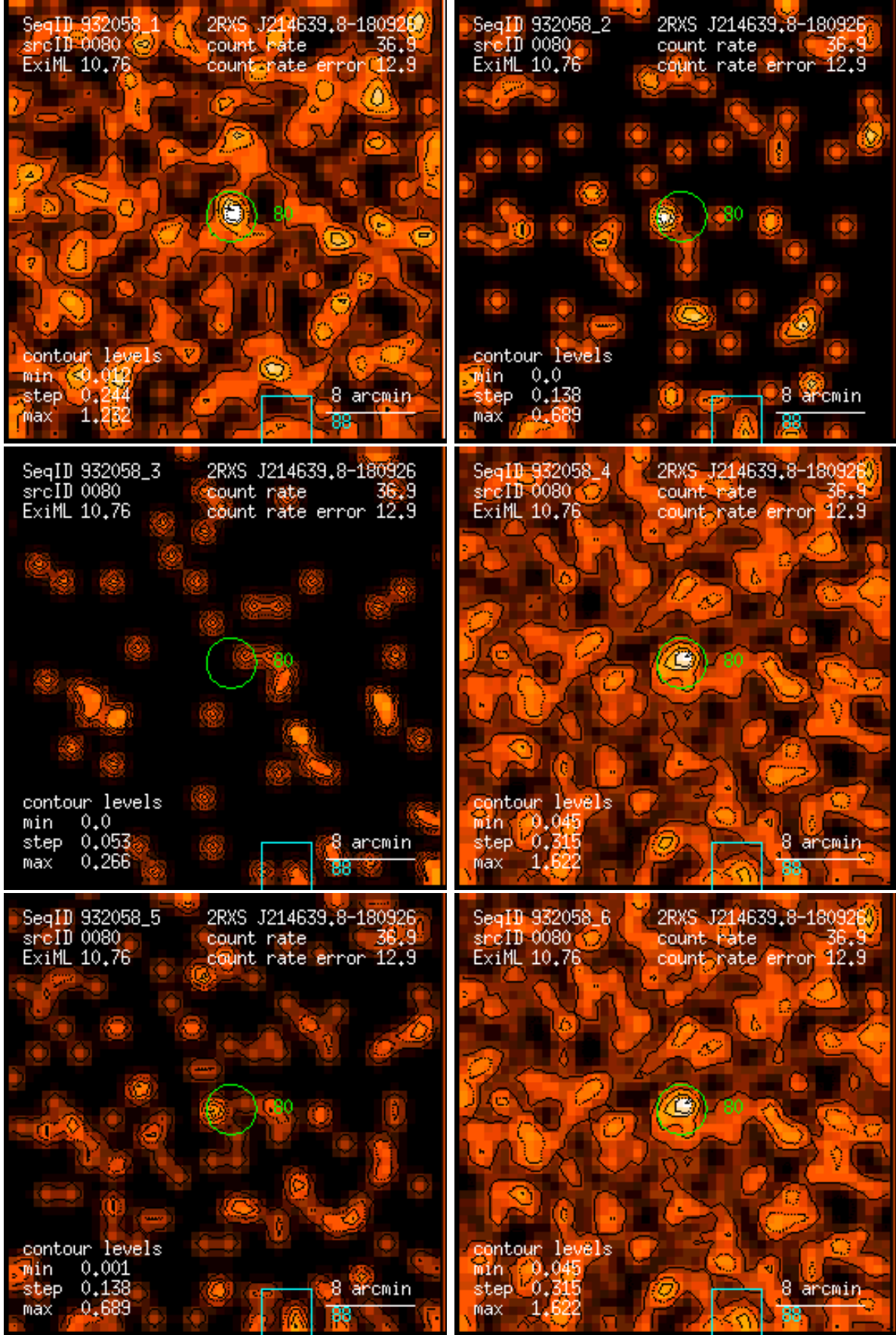
Figure 80: RASS 932058: detection 0080: band rate images, Gaussian filter: (1) PSPC channels 11 – 41, (2) 52 – 90, (3) 91 – 201, (4) 11 – 235, (5) 52 – 201, (6) 11 – 201. Broad band rates in counts/ks. Band rate contour levels in counts/ks/arcmin 2 .
