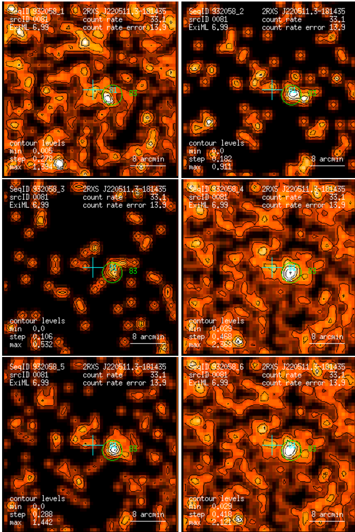
Figure 81: RASS 932058: detection 0081: band rate images, Gaussian filter: (1) PSPC channels 11 – 41, (2) 52 – 90, (3) 91 – 201, (4) 11 – 235, (5) 52 – 201, (6) 11 – 201. Broad band rates in counts/ks. Band rate contour levels in counts/ks/arcmin 2 .
