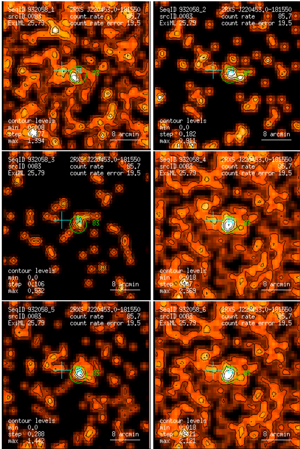
Figure 83: RASS 932058: detection 0083: band rate images, Gaussian filter: (1) PSPC channels 11 – 41, (2) 52 – 90, (3) 91 – 201, (4) 11 – 235, (5) 52 – 201, (6) 11 – 201. Broad band rates in counts/ks. Band rate contour levels in counts/ks/arcmin 2 .
