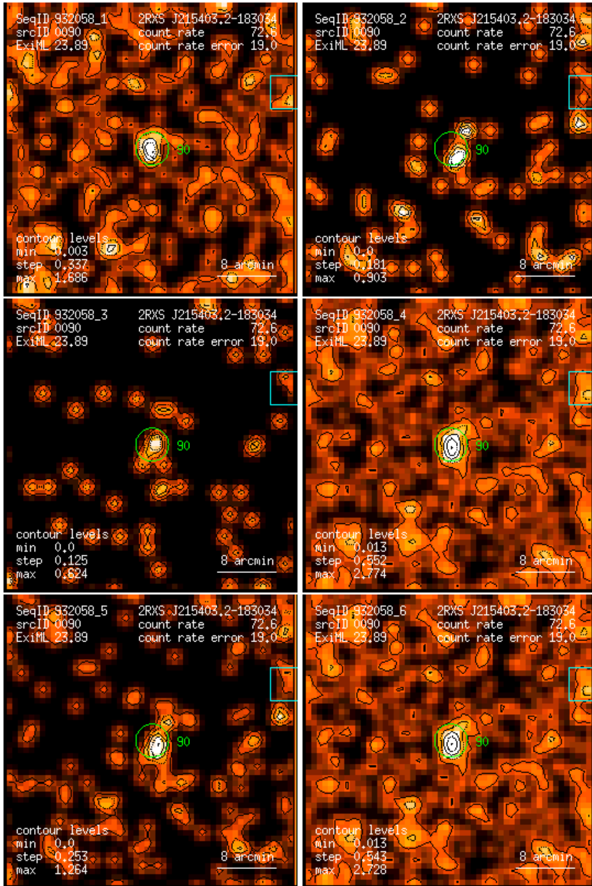
Figure 90: RASS 932058: detection 0090: band rate images, Gaussian filter: (1) PSPC channels 11 – 41, (2) 52 – 90, (3) 91 – 201, (4) 11 – 235, (5) 52 – 201, (6) 11 – 201. Broad band rates in counts/ks. Band rate contour levels in counts/ks/arcmin 2 .
