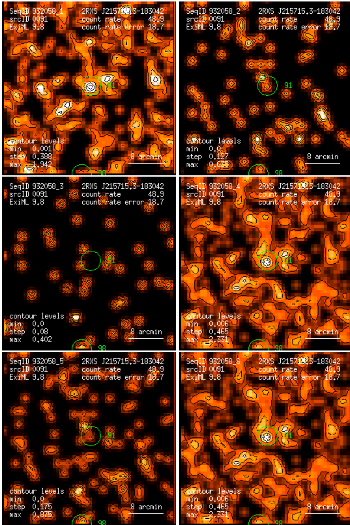
Figure 91: RASS 932058: detection 0091: band rate images, Gaussian filter: (1) PSPC channels 11 – 41, (2) 52 – 90, (3) 91 – 201, (4) 11 – 235, (5) 52 – 201, (6) 11 – 201. Broad band rates in counts/ks. Band rate contour levels in counts/ks/arcmin 2 .
