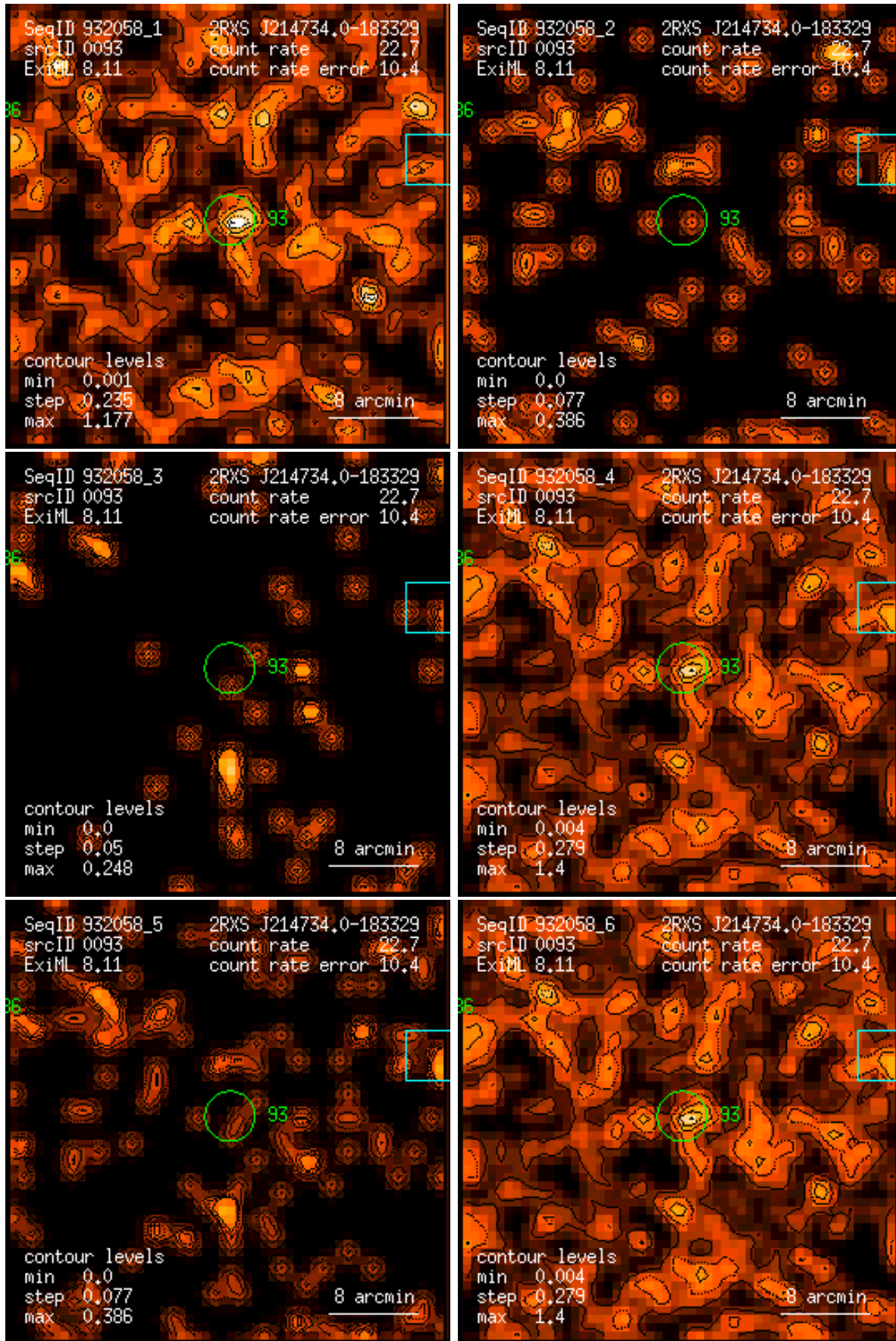
Figure 93: RASS 932058: detection 0093: band rate images, Gaussian filter: (1) PSPC channels 11 – 41, (2) 52 – 90, (3) 91 – 201, (4) 11 – 235, (5) 52 – 201, (6) 11 – 201. Broad band rates in counts/ks. Band rate contour levels in counts/ks/arcmin 2 .
