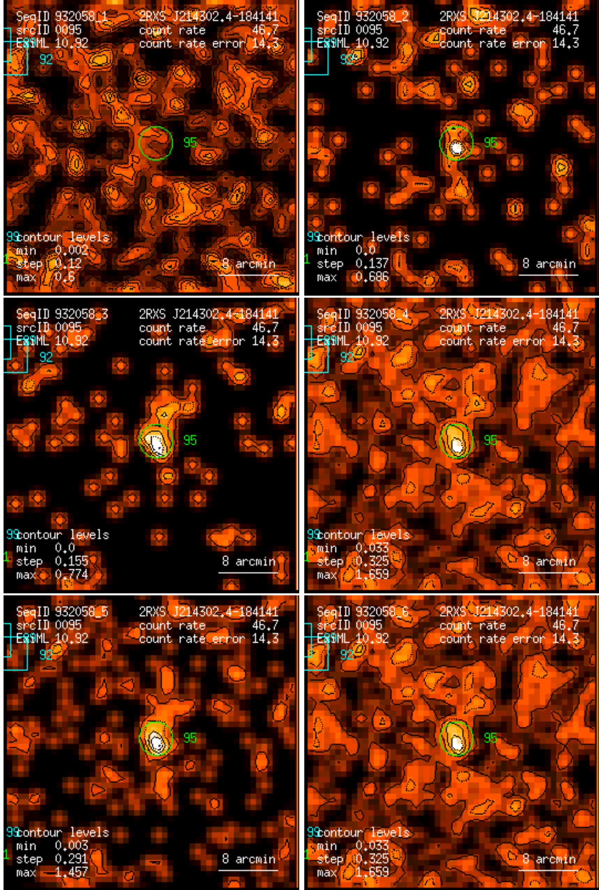
Figure 95: RASS 932058: detection 0095: band rate images, Gaussian filter: (1) PSPC channels 11 – 41, (2) 52 – 90, (3) 91 – 201, (4) 11 – 235, (5) 52 – 201, (6) 11 – 201. Broad band rates in counts/ks. Band rate contour levels in counts/ks/arcmin 2 .
