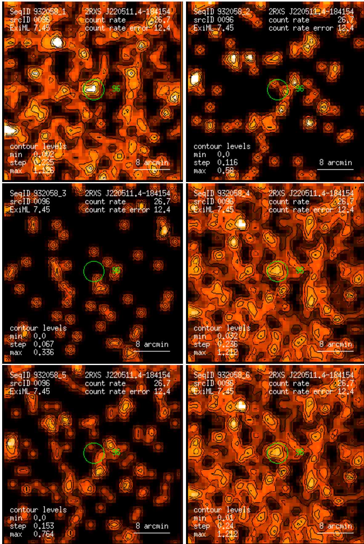
Figure 96: RASS 932058: detection 0096: band rate images, Gaussian filter: (1) PSPC channels 11 – 41, (2) 52 – 90, (3) 91 – 201, (4) 11 – 235, (5) 52 – 201, (6) 11 – 201. Broad band rates in counts/ks. Band rate contour levels in counts/ks/arcmin 2 .
