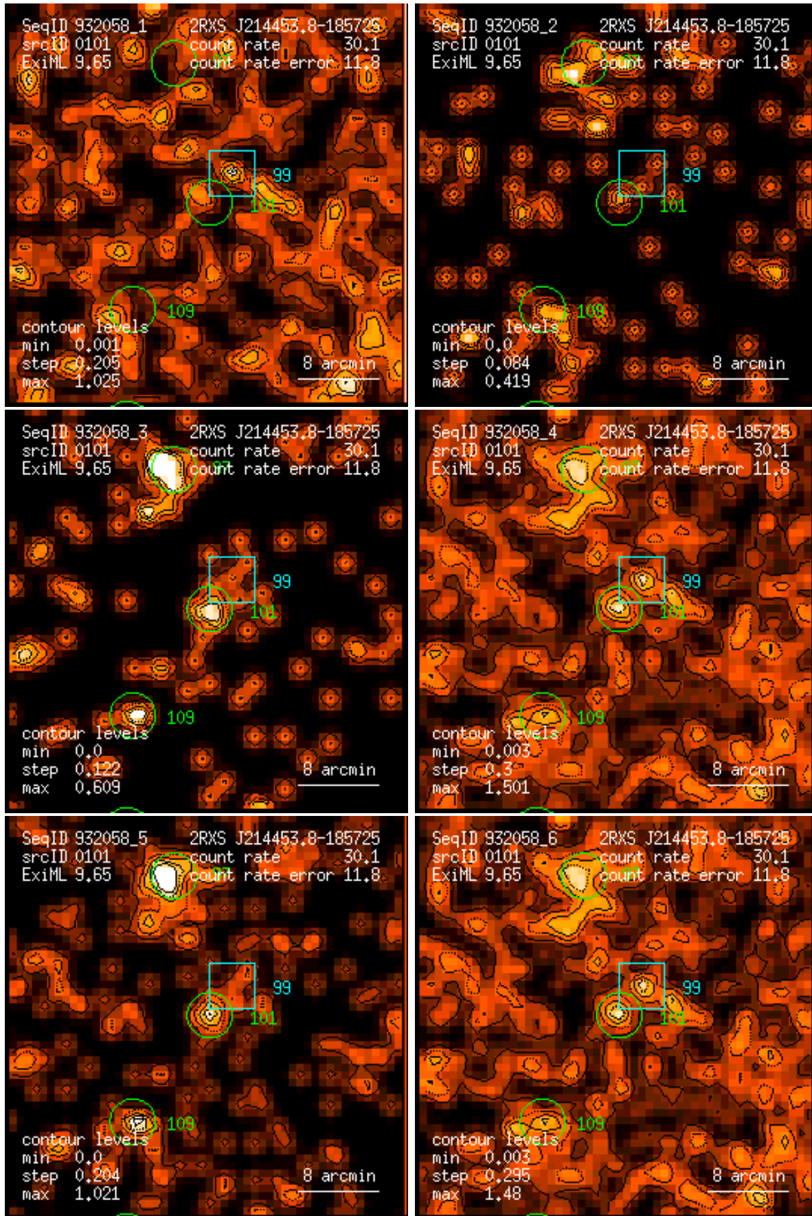
Figure 101: RASS 932058: detection 0101: band rate images, Gaussian filter: (1) PSPC channels 11 – 41, (2) 52 – 90, (3) 91 – 201, (4) 11 – 235, (5) 52 – 201, (6) 11 – 201. Broad band rates in counts/ks. Band rate contour levels in counts/ks/arcmin 2 .
