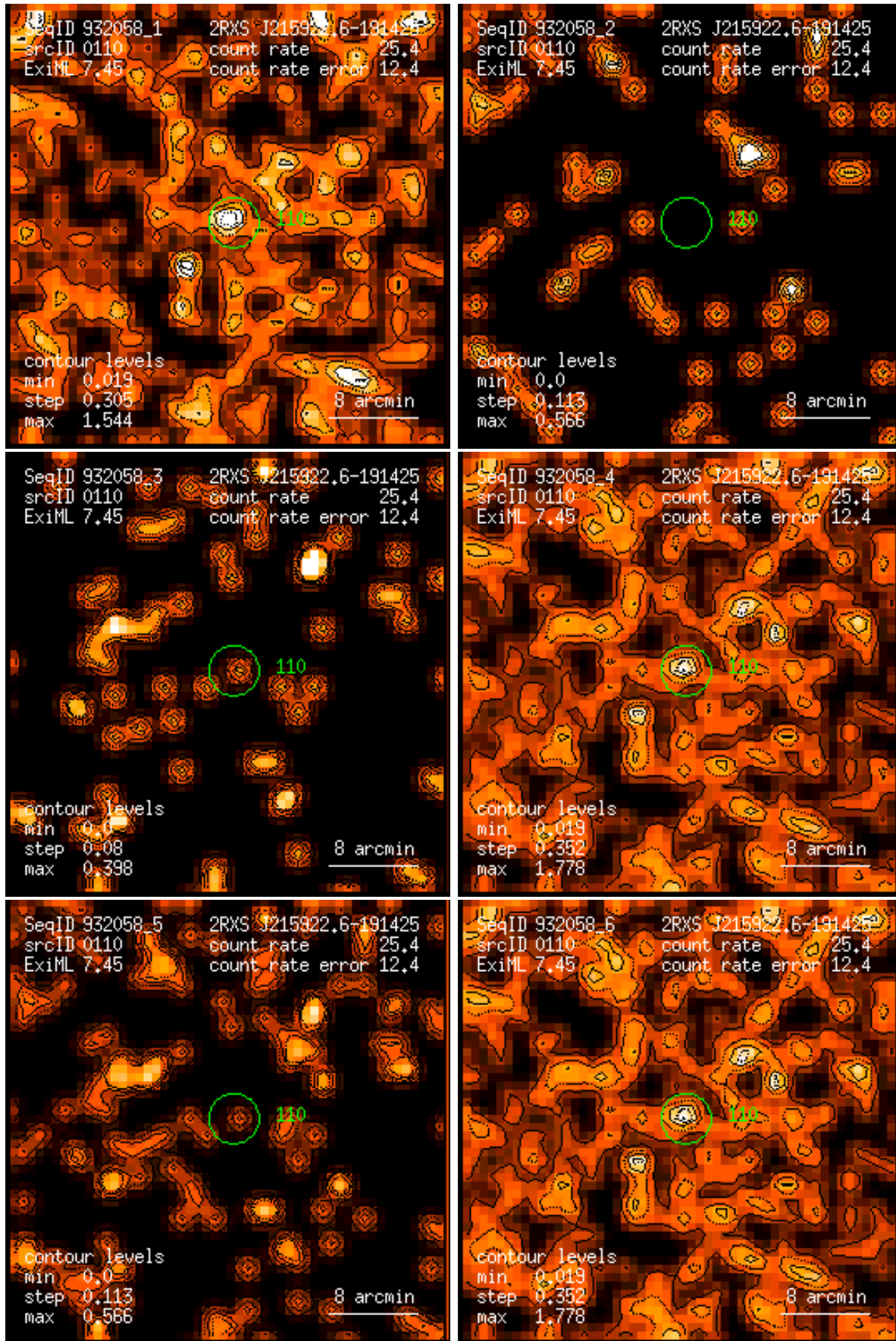
Figure 110: RASS 932058: detection 0110: band rate images, Gaussian filter: (1) PSPC channels 11 – 41, (2) 52 – 90, (3) 91 – 201, (4) 11 – 235, (5) 52 – 201, (6) 11 – 201. Broad band rates in counts/ks. Band rate contour levels in counts/ks/arcmin 2 .
