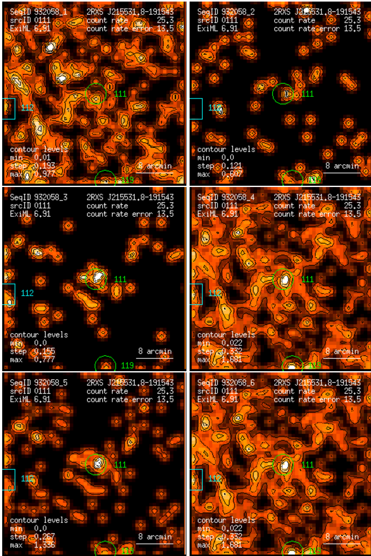
Figure 111: RASS 932058: detection 0111: band rate images, Gaussian filter: (1) PSPC channels 11 – 41, (2) 52 – 90, (3) 91 – 201, (4) 11 – 235, (5) 52 – 201, (6) 11 – 201. Broad band rates in counts/ks. Band rate contour levels in counts/ks/arcmin 2 .
