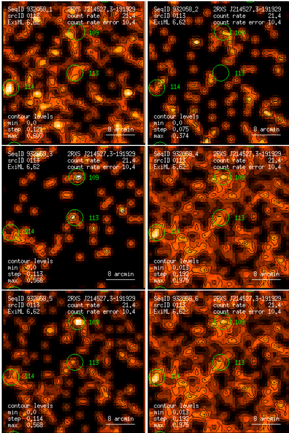
Figure 113: RASS 932058: detection 0113: band rate images, Gaussian filter: (1) PSPC channels 11 – 41, (2) 52 – 90, (3) 91 – 201, (4) 11 – 235, (5) 52 – 201, (6) 11 – 201. Broad band rates in counts/ks. Band rate contour levels in counts/ks/arcmin 2 .
