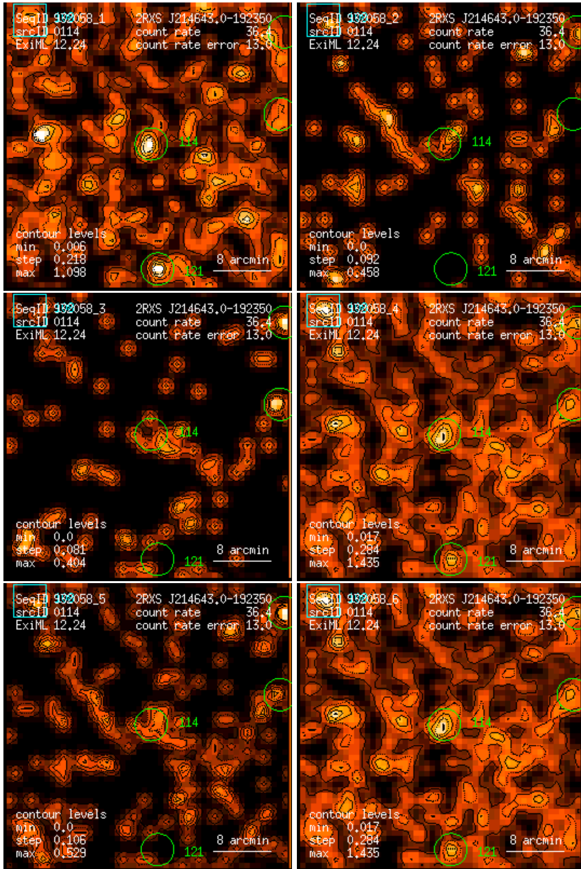
Figure 114: RASS 932058: detection 0114: band rate images, Gaussian filter: (1) PSPC channels 11 – 41, (2) 52 – 90, (3) 91 – 201, (4) 11 – 235, (5) 52 – 201, (6) 11 – 201. Broad band rates in counts/ks. Band rate contour levels in counts/ks/arcmin 2 .
