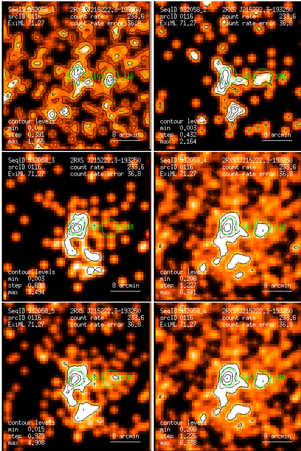
Figure 116: RASS 932058: detection 0116: band rate images, Gaussian filter: (1) PSPC channels 11 – 41, (2) 52 – 90, (3) 91 – 201, (4) 11 – 235, (5) 52 – 201, (6) 11 – 201. Broad band rates in counts/ks. Band rate contour levels in counts/ks/arcmin 2 .
