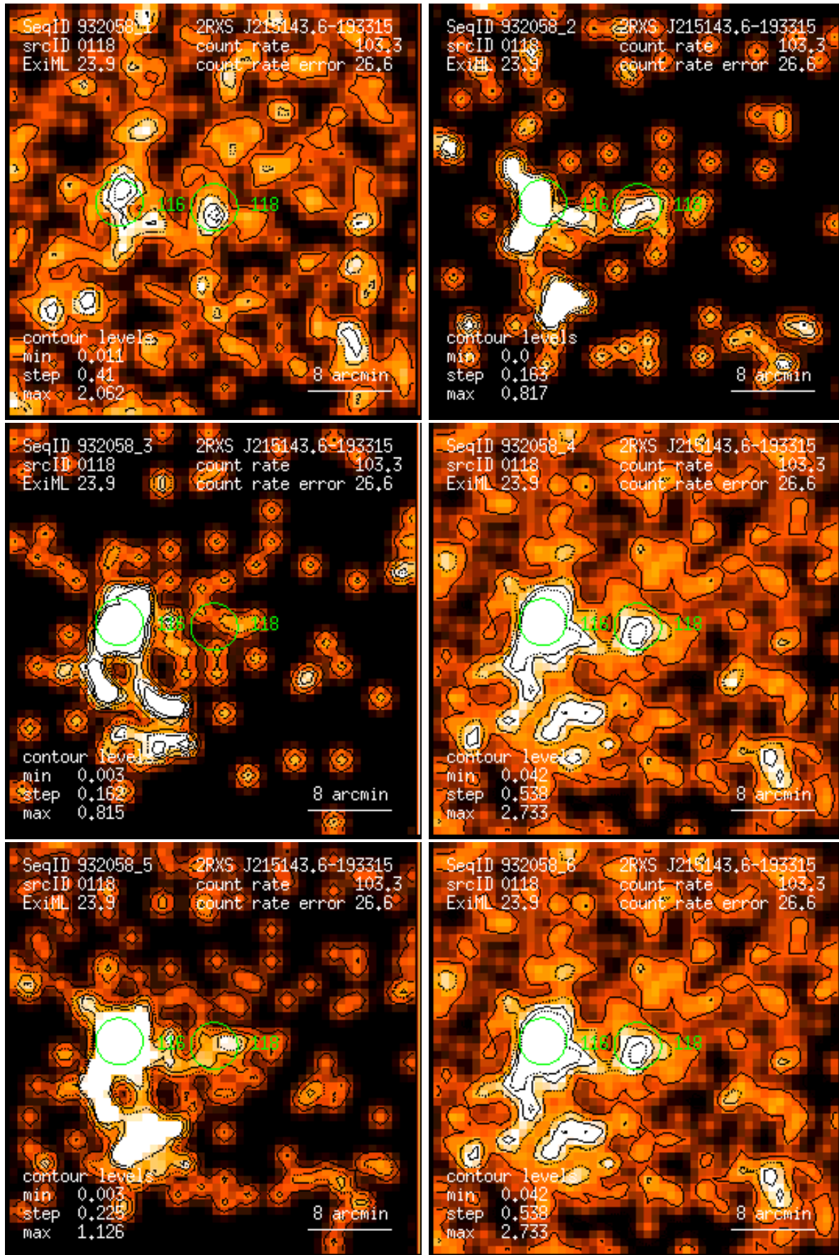
Figure 118: RASS 932058: detection 0118: band rate images, Gaussian filter: (1) PSPC channels 11 – 41, (2) 52 – 90, (3) 91 – 201, (4) 11 – 235, (5) 52 – 201, (6) 11 – 201. Broad band rates in counts/ks. Band rate contour levels in counts/ks/arcmin 2 .
