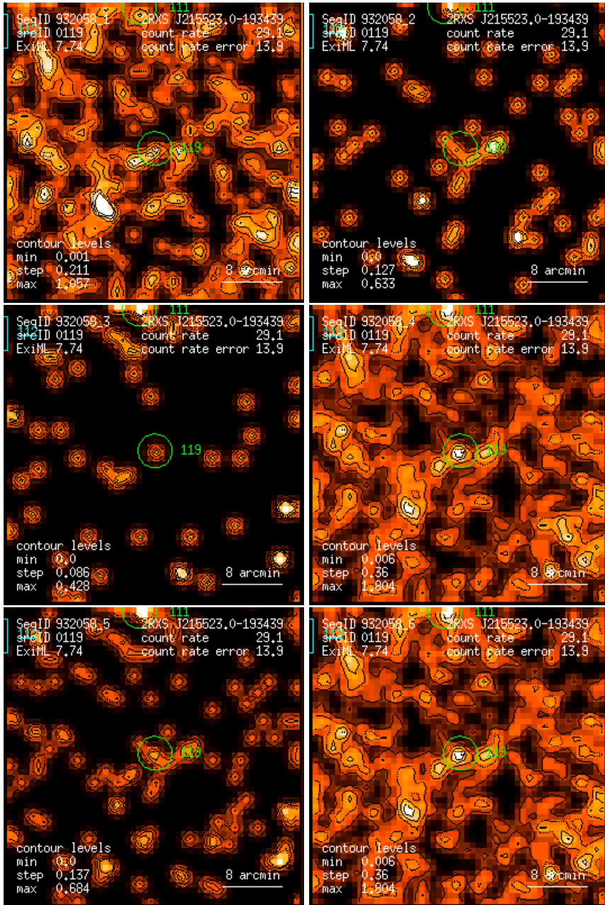
Figure 119: RASS 932058: detection 0119: band rate images, Gaussian filter: (1) PSPC channels 11 – 41, (2) 52 – 90, (3) 91 – 201, (4) 11 – 235, (5) 52 – 201, (6) 11 – 201. Broad band rates in counts/ks. Band rate contour levels in counts/ks/arcmin 2 .
