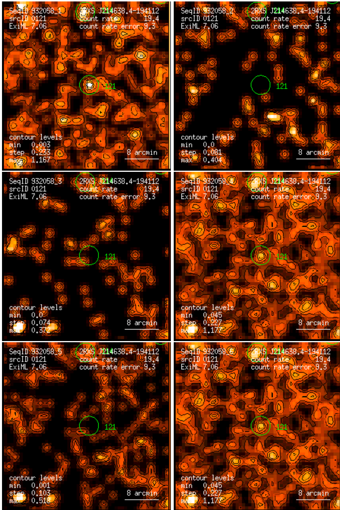
Figure 121: RASS 932058: detection 0121: band rate images, Gaussian filter: (1) PSPC channels 11 – 41, (2) 52 – 90, (3) 91 – 201, (4) 11 – 235, (5) 52 – 201, (6) 11 – 201. Broad band rates in counts/ks. Band rate contour levels in counts/ks/arcmin 2 .
