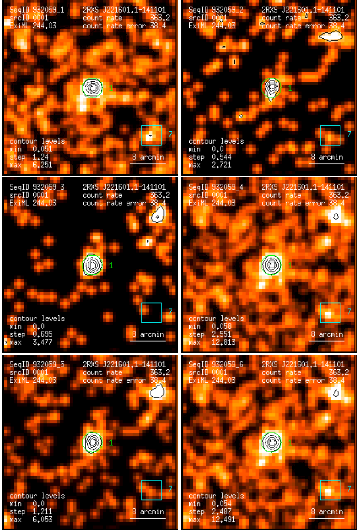
Figure 1: RASS 932059: detection 0001: band rate images, Gaussian filter: (1) PSPC channels 11 – 41, (2) 52 – 90, (3) 91 – 201, (4) 11 – 235, (5) 52 – 201, (6) 11 – 201. Broad band rates in counts/ks. Band rate contour levels in counts/ks/arcmin 2 .
