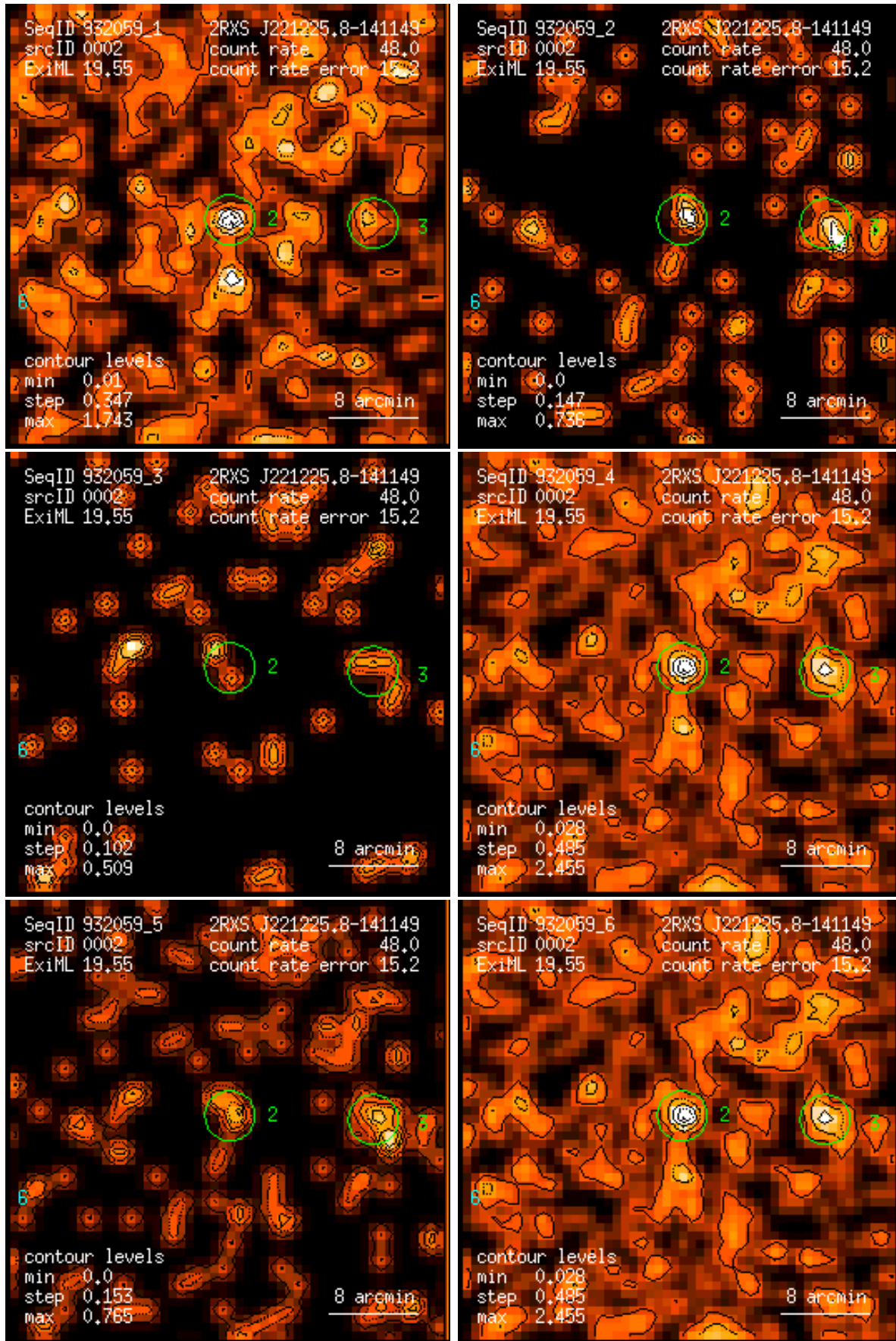
Figure 2: RASS 932059: detection 0002: band rate images, Gaussian filter: (1) PSPC channels 11 – 41, (2) 52 – 90, (3) 91 – 201, (4) 11 – 235, (5) 52 – 201, (6) 11 – 201. Broad band rates in counts/ks. Band rate contour levels in counts/ks/arcmin 2 .
