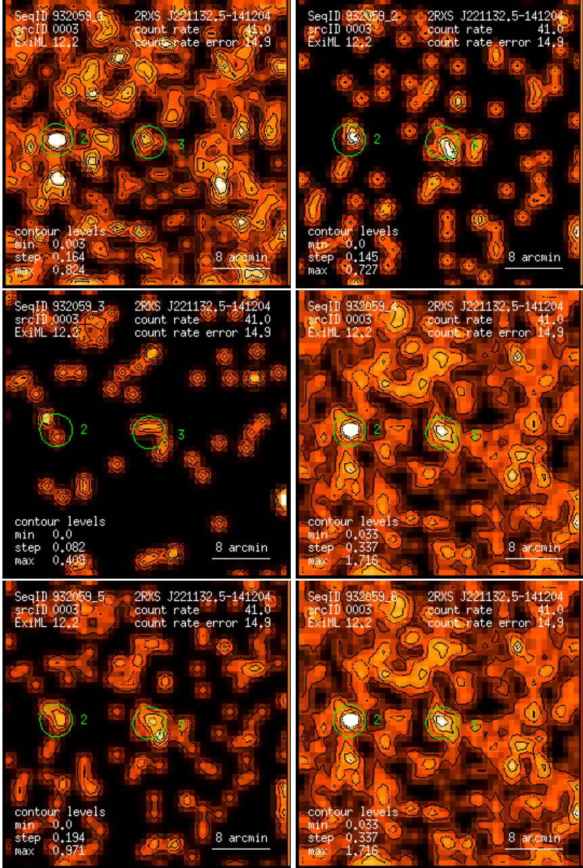
Figure 3: RASS 932059: detection 0003: band rate images, Gaussian filter: (1) PSPC channels 11 – 41, (2) 52 – 90, (3) 91 – 201, (4) 11 – 235, (5) 52 – 201, (6) 11 – 201. Broad band rates in counts/ks. Band rate contour levels in counts/ks/arcmin 2 .
