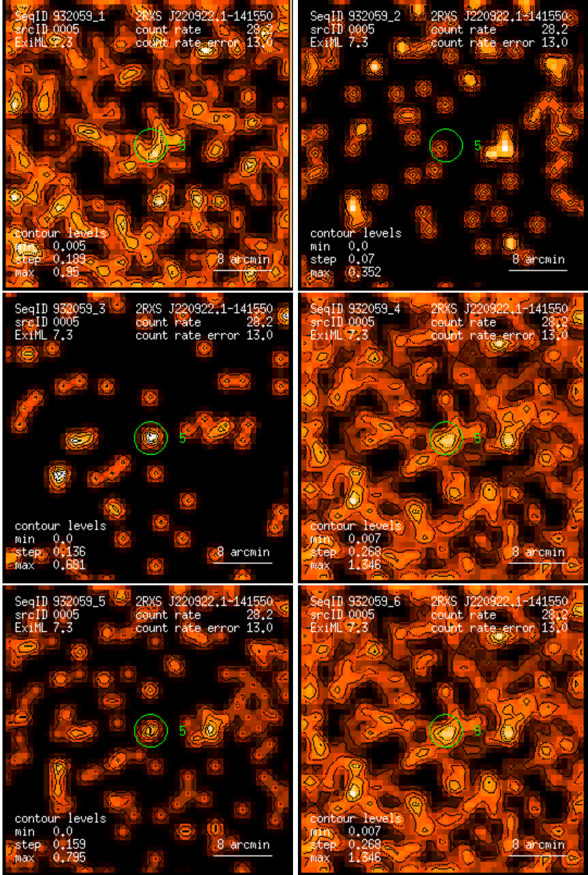
Figure 5: RASS 932059: detection 0005: band rate images, Gaussian filter: (1) PSPC channels 11 – 41, (2) 52 – 90, (3) 91 – 201, (4) 11 – 235, (5) 52 – 201, (6) 11 – 201. Broad band rates in counts/ks. Band rate contour levels in counts/ks/arcmin 2 .
