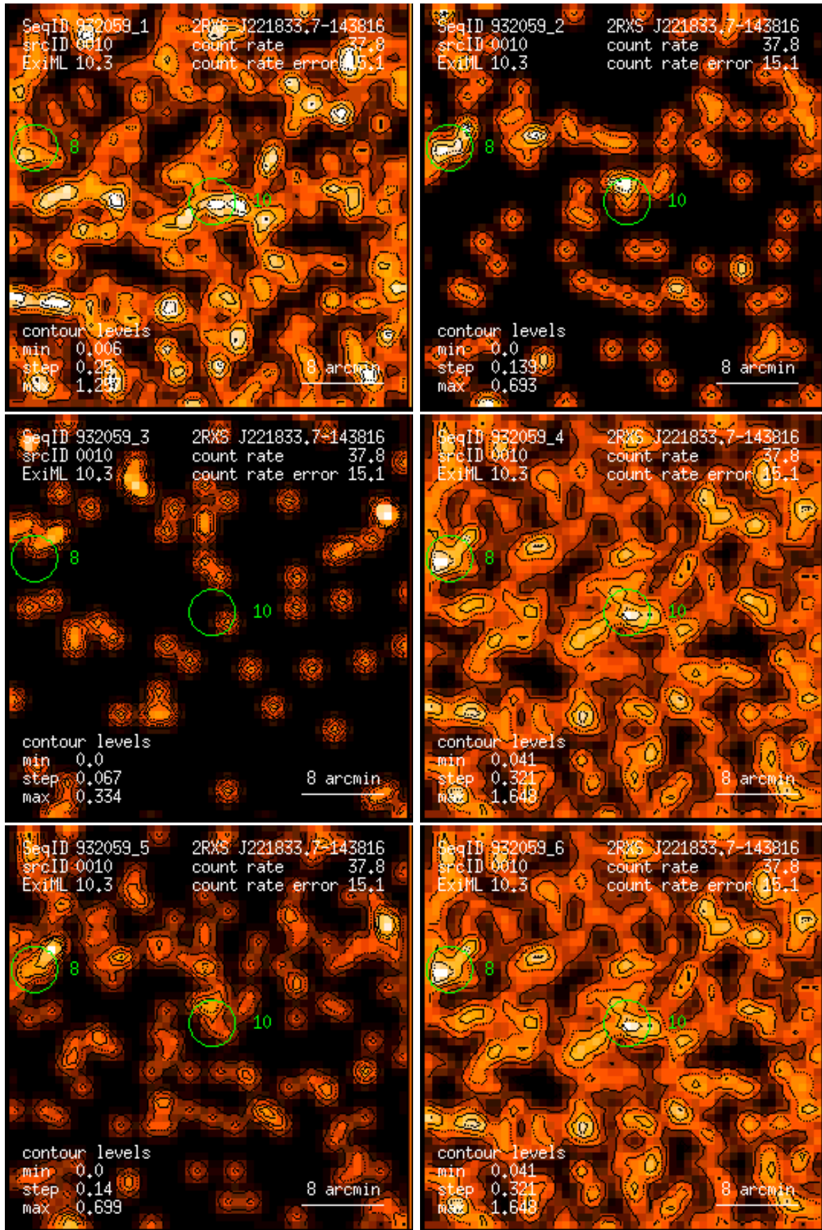
Figure 10: RASS 932059: detection 0010: band rate images, Gaussian filter: (1) PSPC channels 11 – 41, (2) 52 – 90, (3) 91 – 201, (4) 11 – 235, (5) 52 – 201, (6) 11 – 201. Broad band rates in counts/ks. Band rate contour levels in counts/ks/arcmin 2 .
