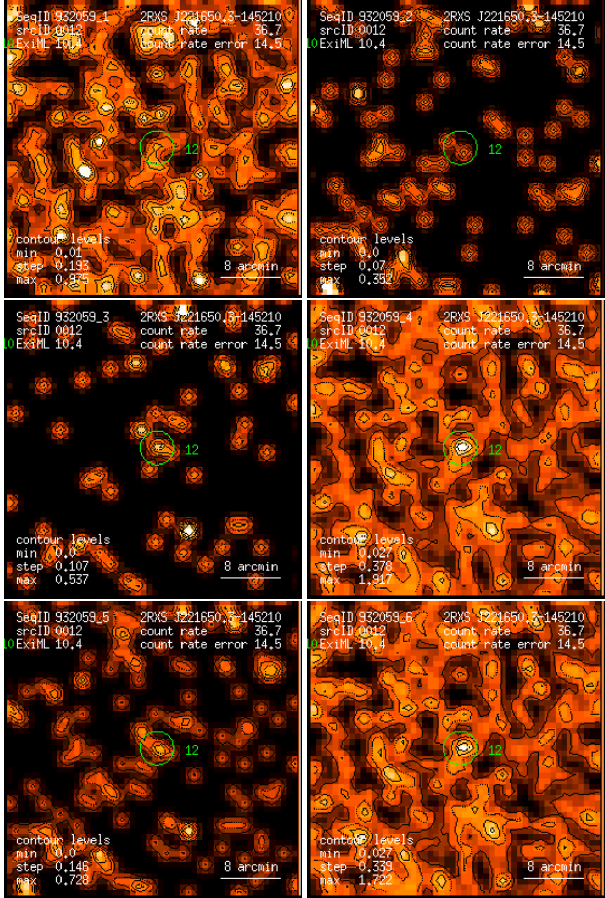
Figure 12: RASS 932059: detection 0012: band rate images, Gaussian filter: (1) PSPC channels 11 – 41, (2) 52 – 90, (3) 91 – 201, (4) 11 – 235, (5) 52 – 201, (6) 11 – 201. Broad band rates in counts/ks. Band rate contour levels in counts/ks/arcmin 2 .
