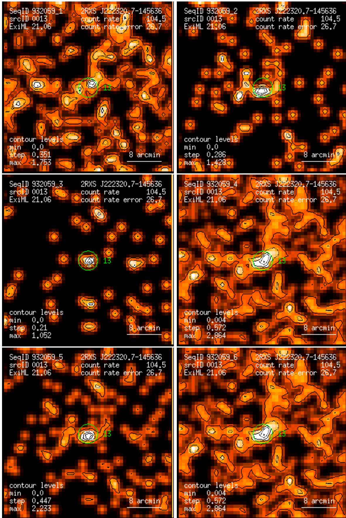
Figure 13: RASS 932059: detection 0013: band rate images, Gaussian filter: (1) PSPC channels 11 – 41, (2) 52 – 90, (3) 91 – 201, (4) 11 – 235, (5) 52 – 201, (6) 11 – 201. Broad band rates in counts/ks. Band rate contour levels in counts/ks/arcmin 2 .
