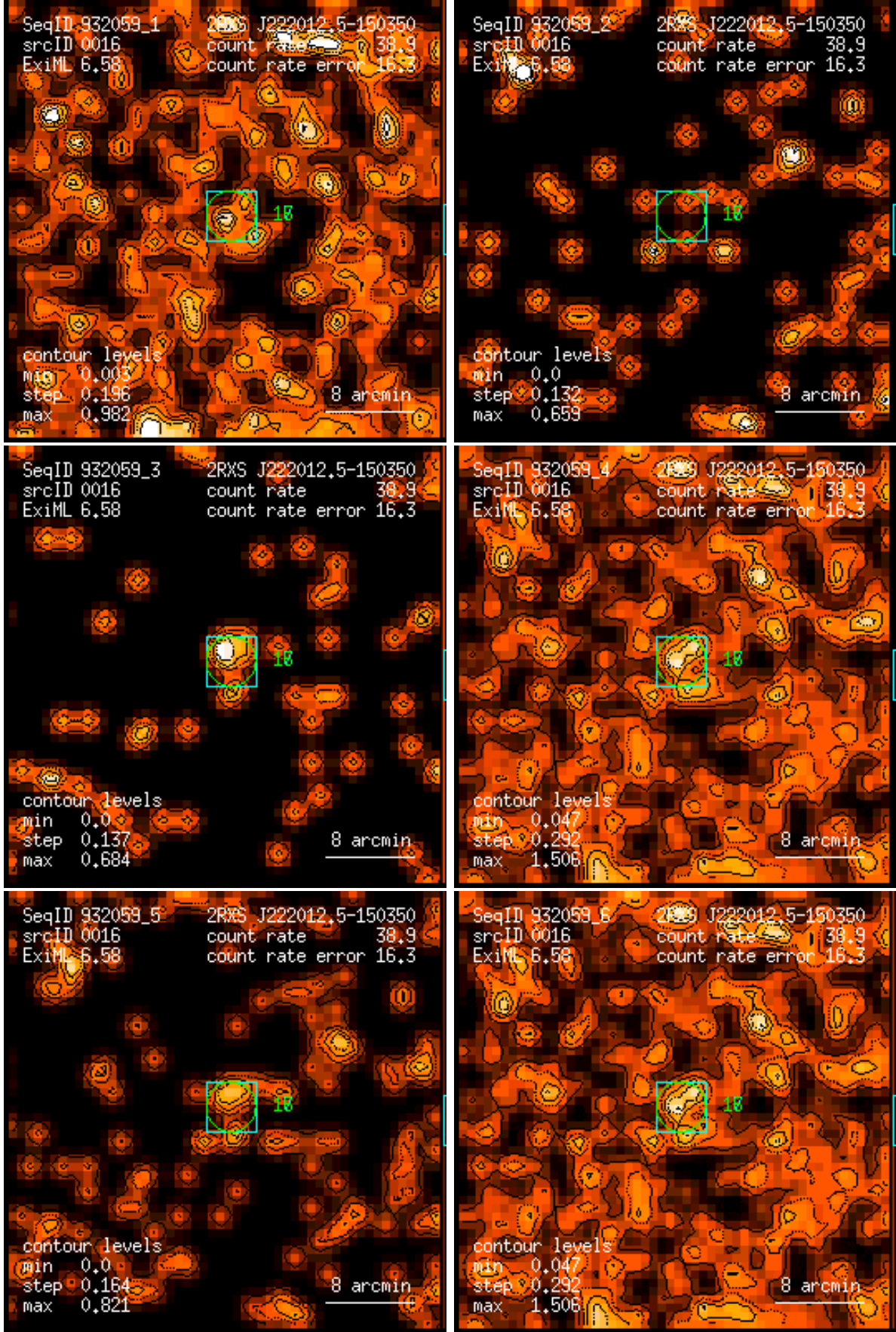
Figure 16: RASS 932059: detection 0016: band rate images, Gaussian filter: (1) PSPC channels 11 – 41, (2) 52 – 90, (3) 91 – 201, (4) 11 – 235, (5) 52 – 201, (6) 11 – 201. Broad band rates in counts/ks. Band rate contour levels in counts/ks/arcmin 2 .
