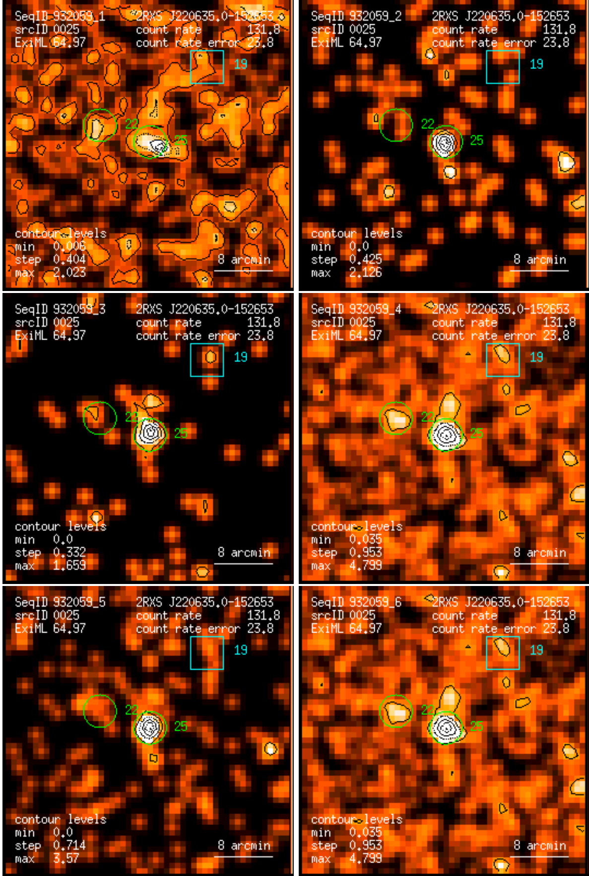
Figure 25: RASS 932059: detection 0025: band rate images, Gaussian filter: (1) PSPC channels 11 – 41, (2) 52 – 90, (3) 91 – 201, (4) 11 – 235, (5) 52 – 201, (6) 11 – 201. Broad band rates in counts/ks. Band rate contour levels in counts/ks/arcmin 2 .
