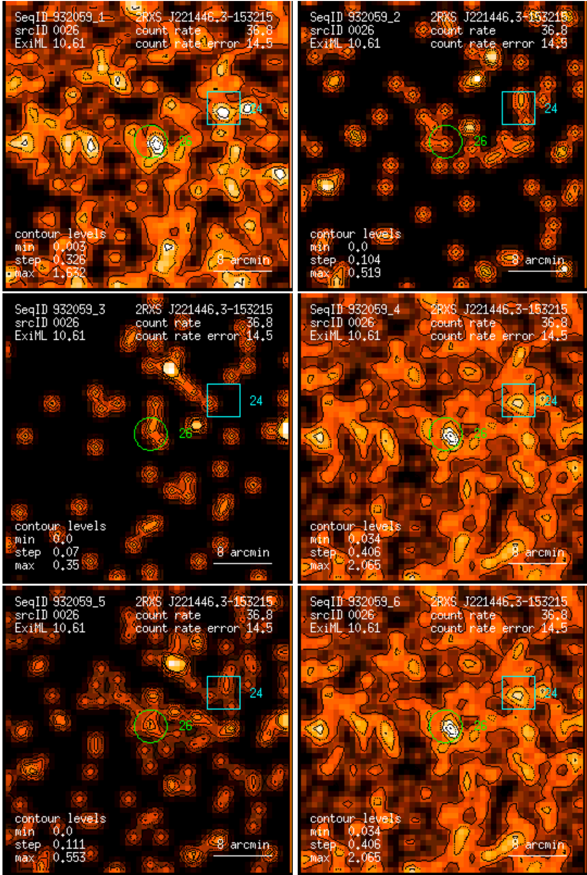
Figure 26: RASS 932059: detection 0026: band rate images, Gaussian filter: (1) PSPC channels 11 – 41, (2) 52 – 90, (3) 91 – 201, (4) 11 – 235, (5) 52 – 201, (6) 11 – 201. Broad band rates in counts/ks. Band rate contour levels in counts/ks/arcmin 2 .
