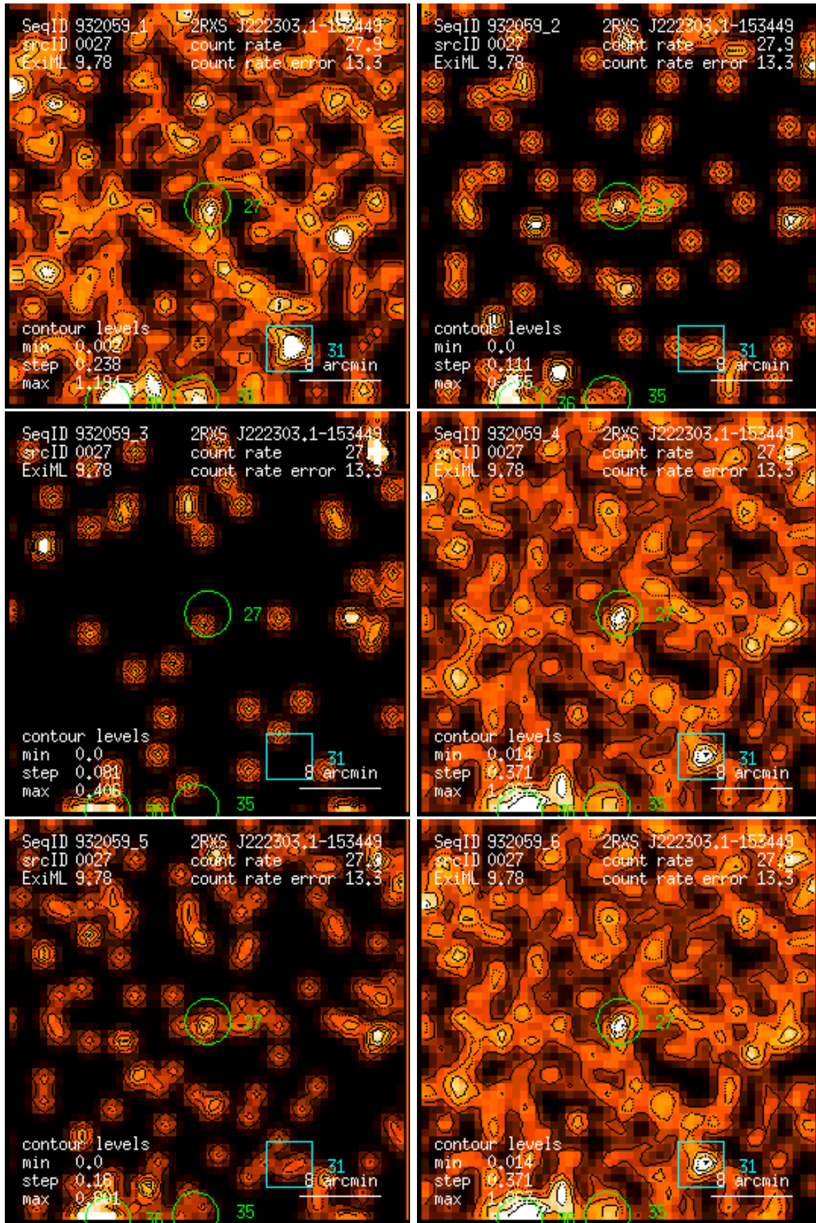
Figure 27: RASS 932059: detection 0027: band rate images, Gaussian filter: (1) PSPC channels 11 – 41, (2) 52 – 90, (3) 91 – 201, (4) 11 – 235, (5) 52 – 201, (6) 11 – 201. Broad band rates in counts/ks. Band rate contour levels in counts/ks/arcmin 2 .
